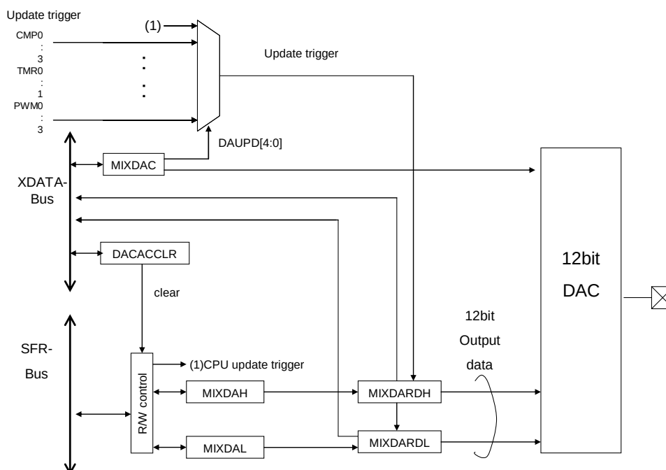
Figure 23-1 Block diagram of 12bit DAC
