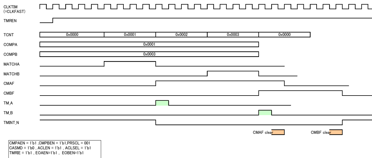
Figure 16-2 Compare match timing Chart
