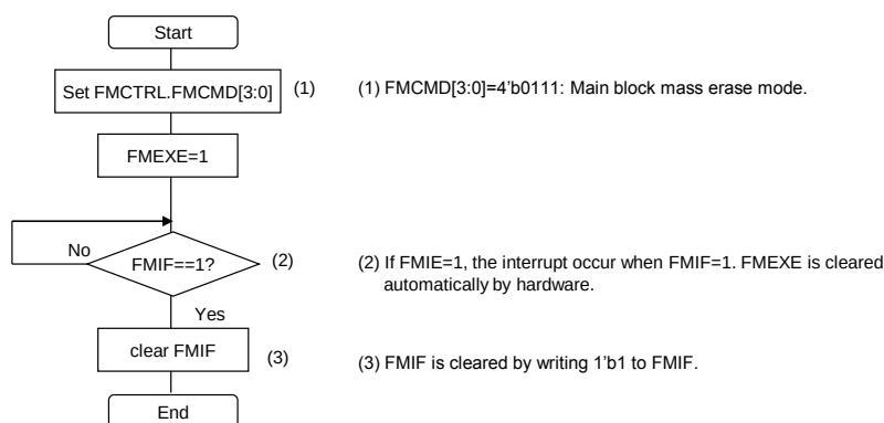
Figure 12-3 Mass erase operation sequence
