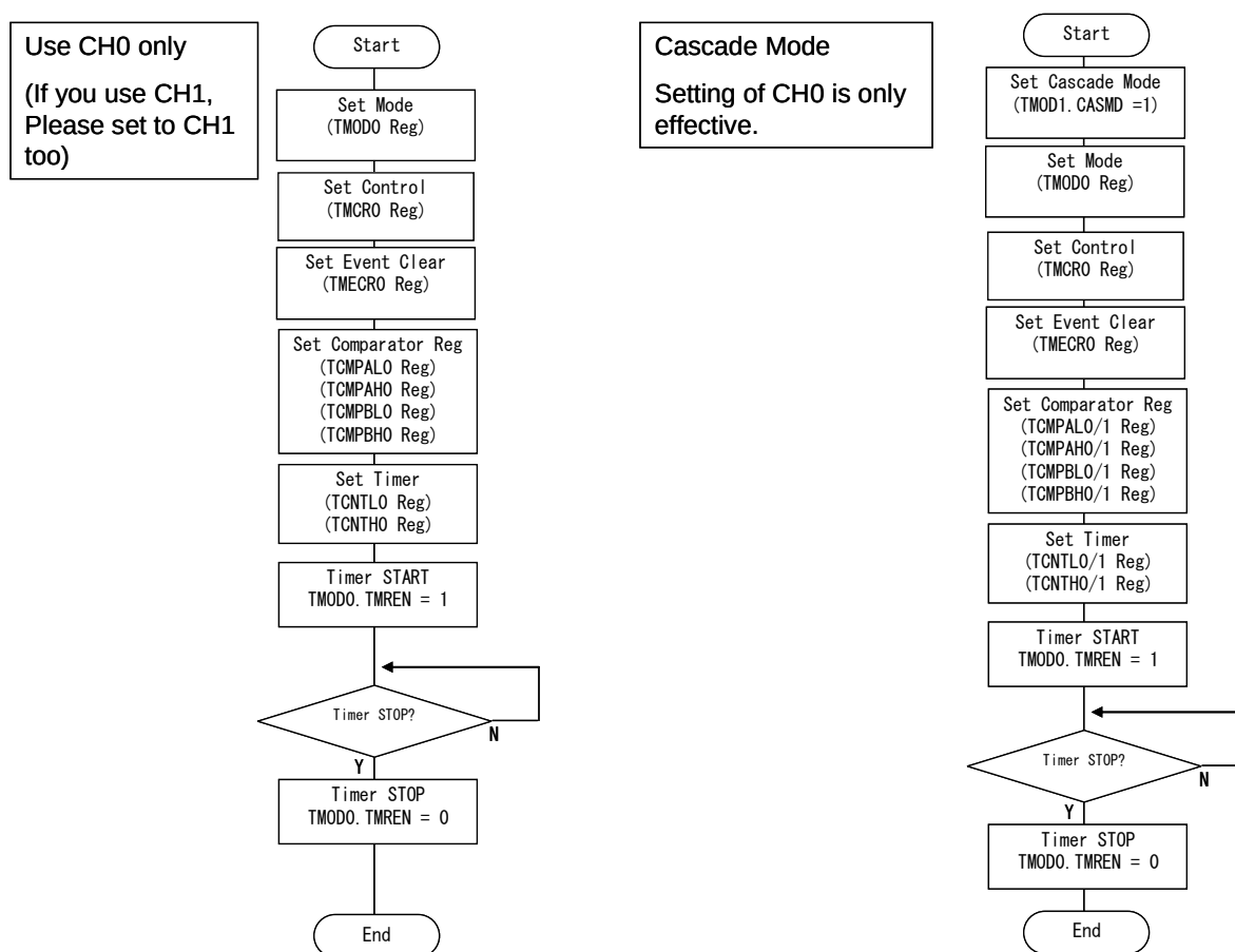
Figure 16-3 Flow Chart
