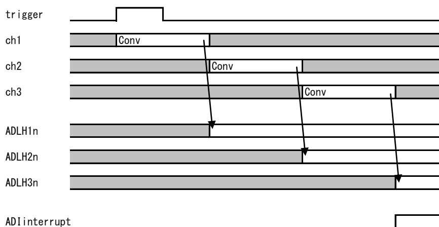
Figure 22-3 Burst until Sequence End mode.
