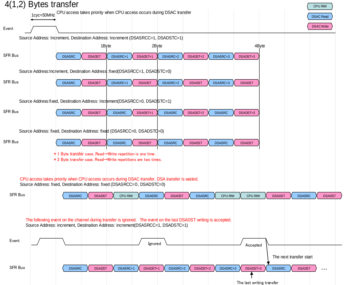
Figure 11-2 4(1,2) Bytes transfer
