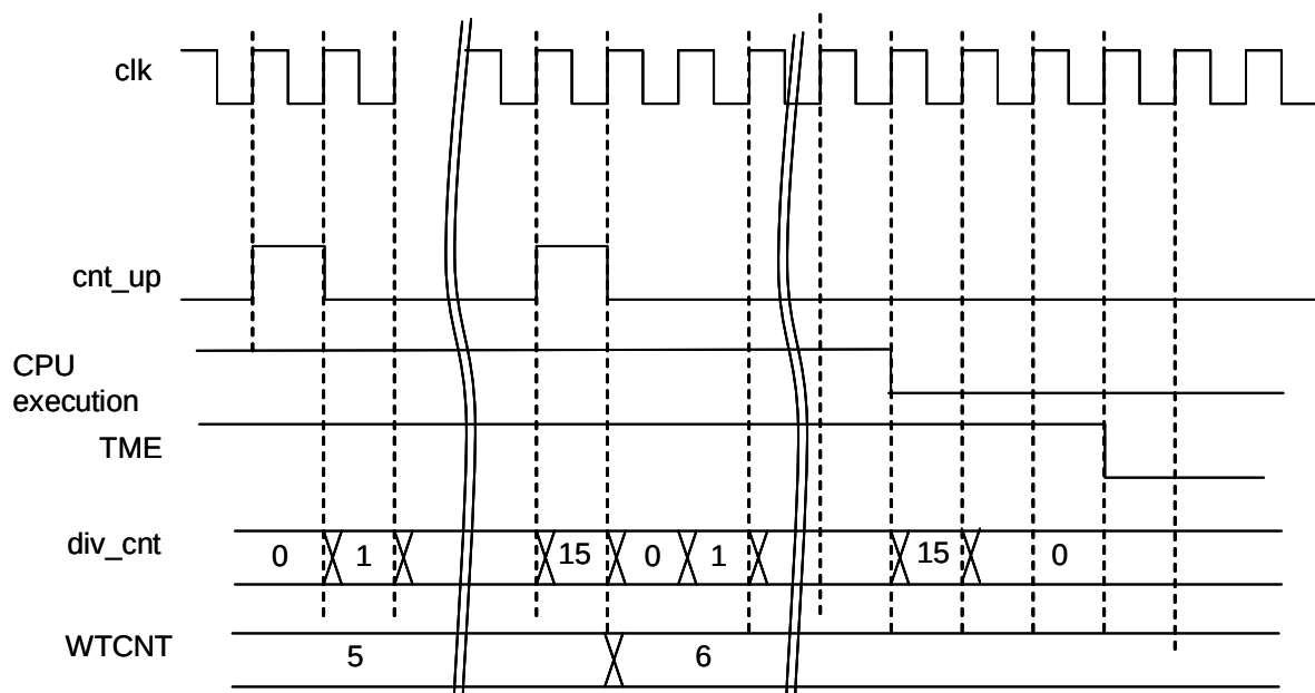
Figure 15-5 Prescaler operation
