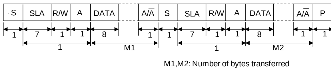
Figure 18-6 I2C bus data format
