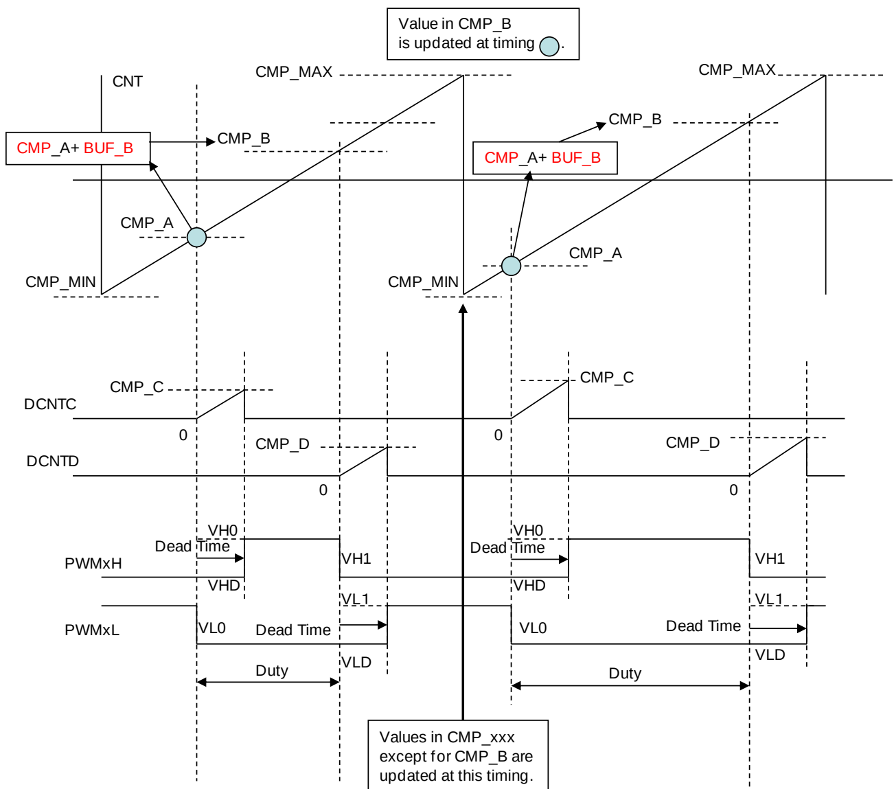
Figure 14-8 PWM Mode 3 (Phase Shift, Auto Dead Time Mode 0)
