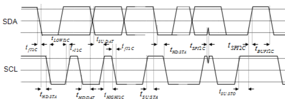
Figure 29-4 I2C timing
