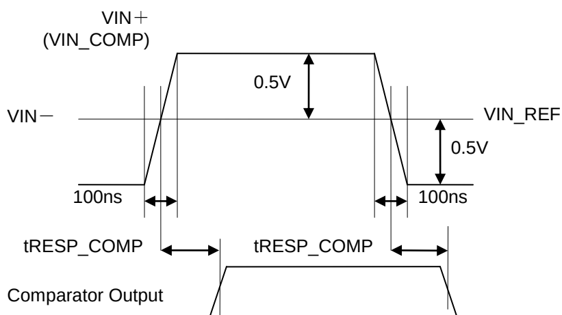
Figure 29-1 Comparator Timing Chart
