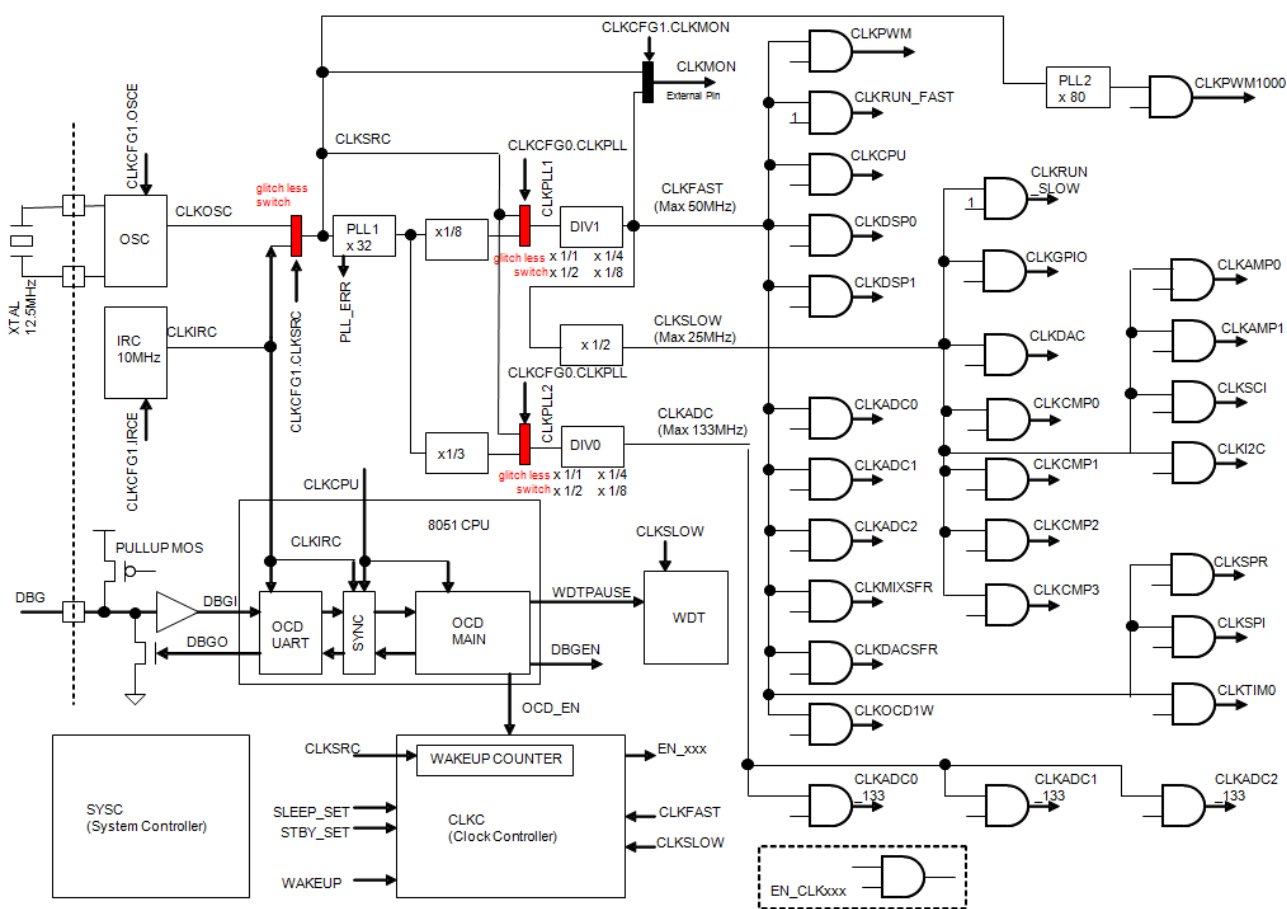
Figure 5-1 Clock System
