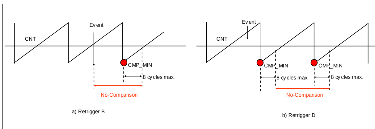
Figure 14-21 No-Comparison period
