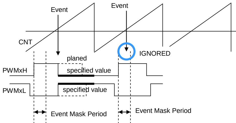
Figure 14-19 Re-Trigger Operation D
