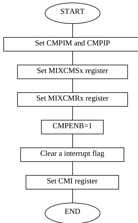
Figure 25-3 Operation flowchart
