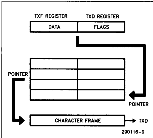
Figure 9. Tx FIFO
