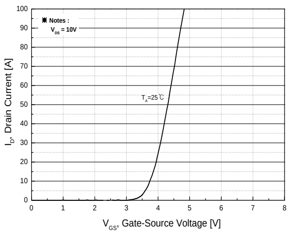
Fig.5 Transfer Characteristics
