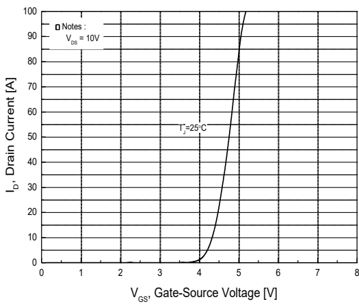
Fig.5 Transfer Characteristics
