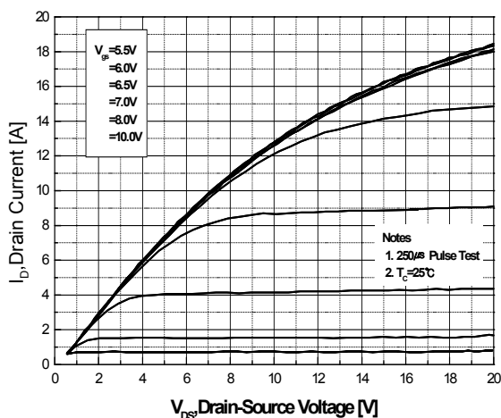
Fig.1 On-Region Characteristics
