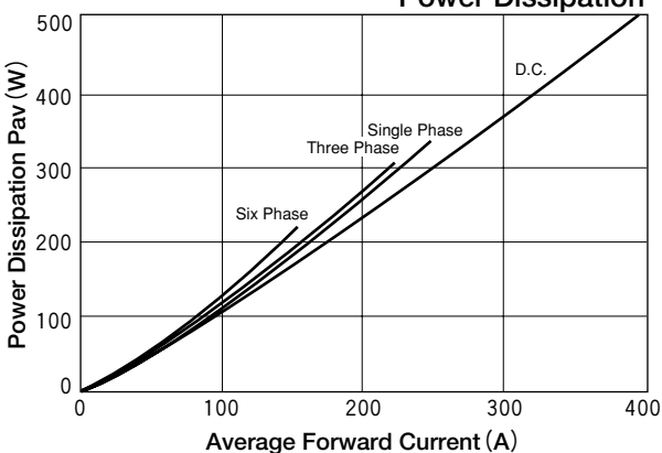
Average Forward Current vs. Power Dissipation
