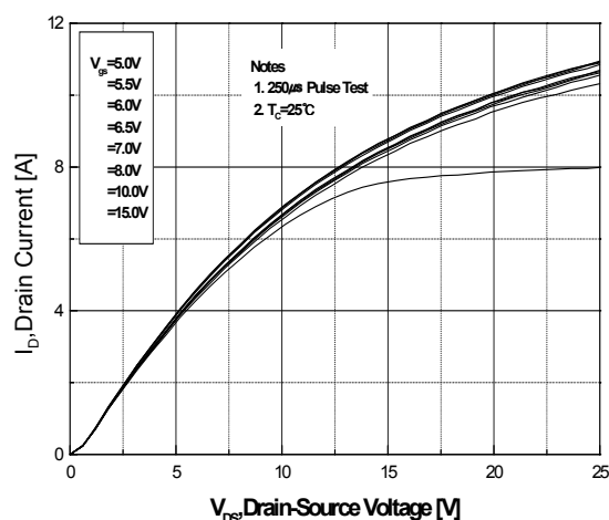
Fig.1 On-Region Characteristics
