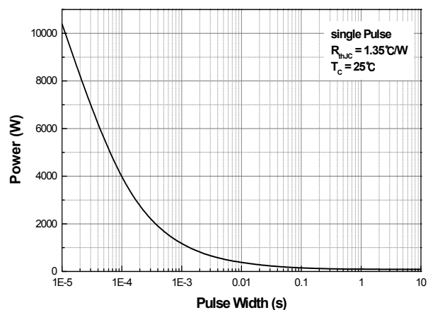
Fig.12 Single Pulse Maximum Power Dissipation – MDP5N50B (TO-220)
