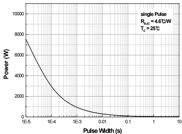
Fig.14 Single Pulse Maximum Power Dissipation – MDF5N50B (TO-220F)
