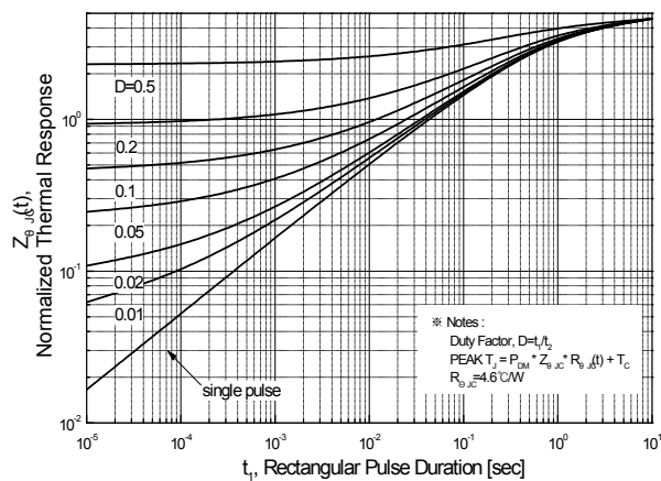
Fig.15 Transient Thermal Response Curve MDF5N50B (TO-220F)
