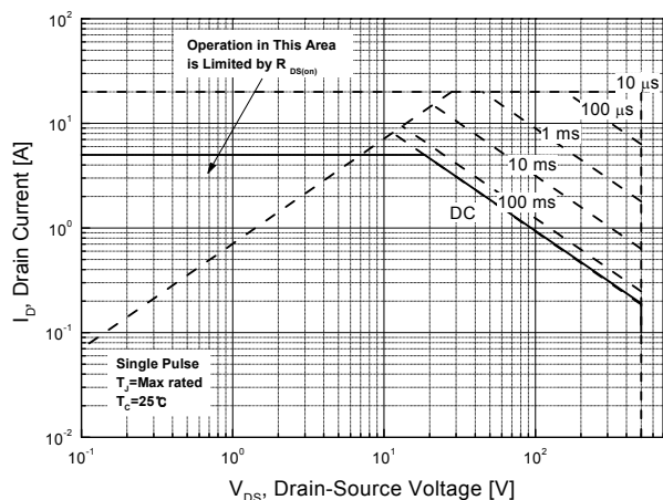
Fig.9 Maximum Safe Operating Area MDP5N50B (TO-220)
