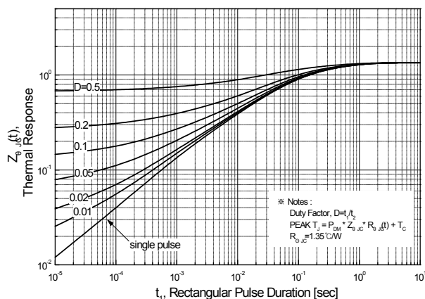
Fig.11 Transient Thermal Response Curve MDP5N50B (TO-220)
