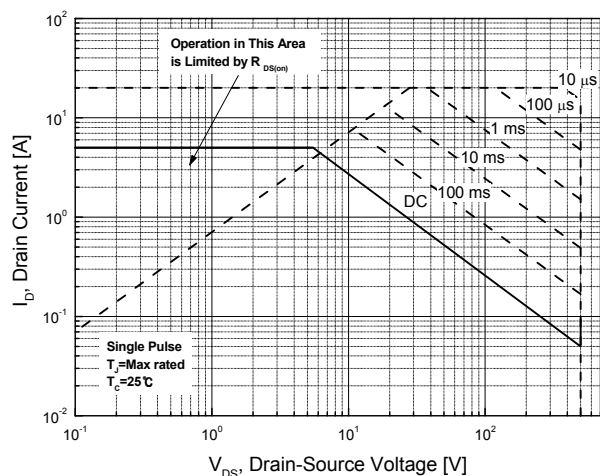
Fig.13 Maximum Safe Operating Area MDF5N50B (TO-220F)
