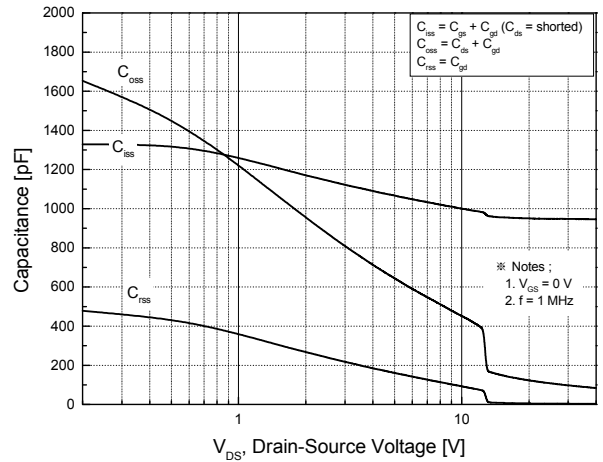
Fig.8 Capacitance Characteristics
