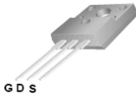
TO-220FS MDFS Series
