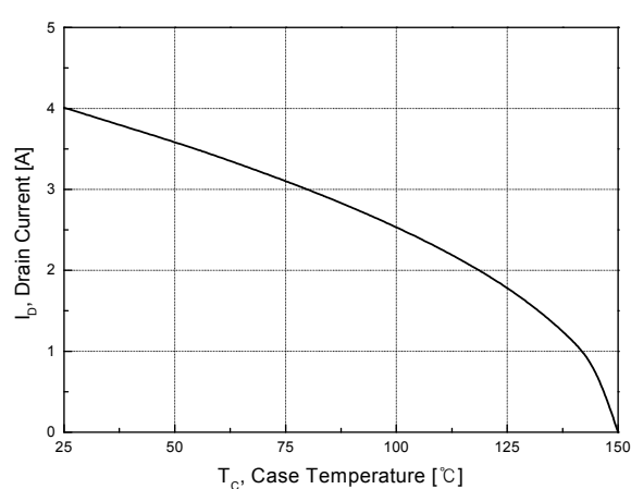
Fig.15 Maximum Drain Current vs. Case Temperature
