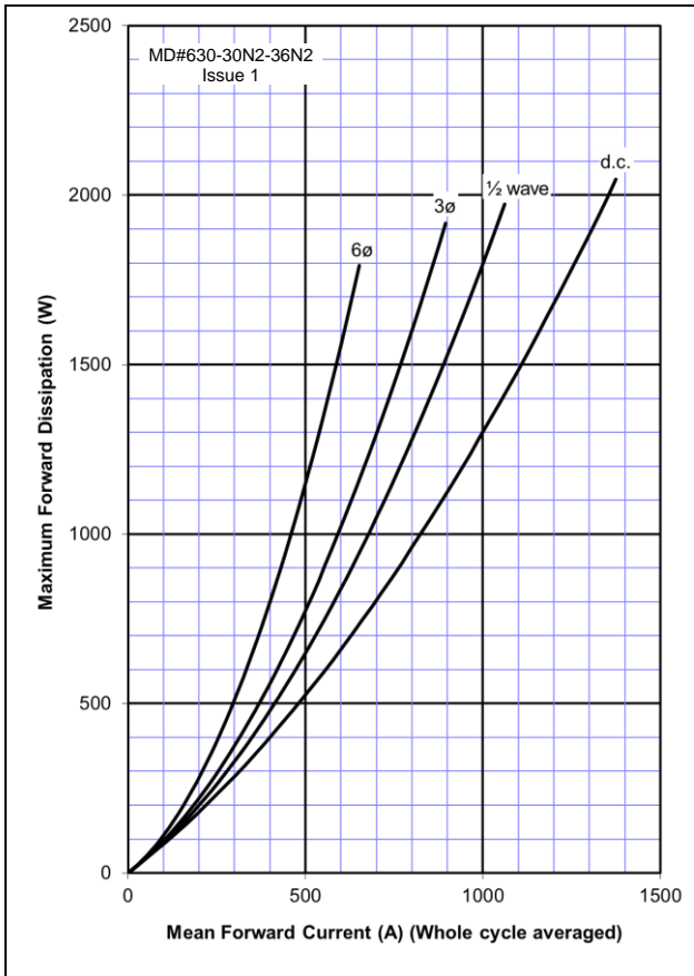
Figure 7 – Forward current vs. Power dissipation
