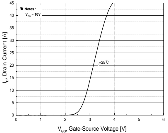
Fig.5 Transfer Characteristics
