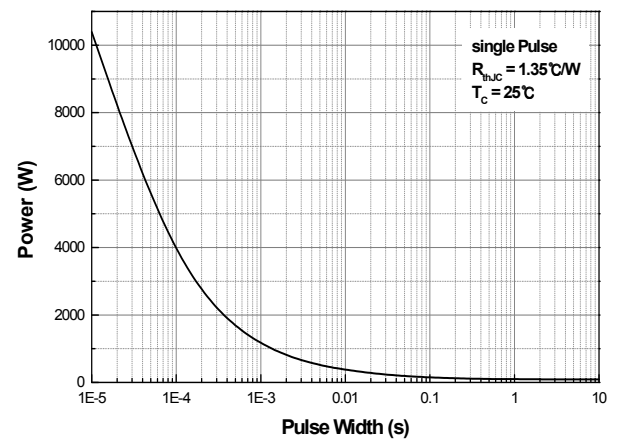
Fig.12 Single Pulse Maximum Power Dissipation – MDP5N50B (TO-220)
