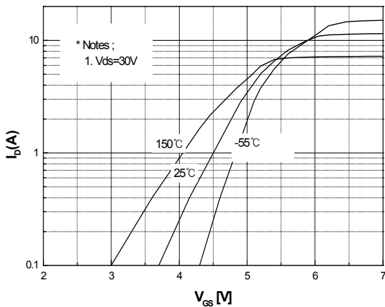
Fig.5 Transfer Characteristics
