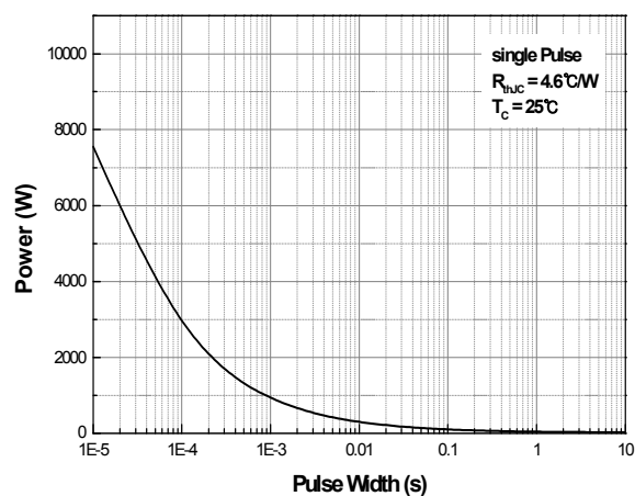
Fig.12 Single Pulse Maximum Power Dissipation- MDF5N50Z (TO-220F)
