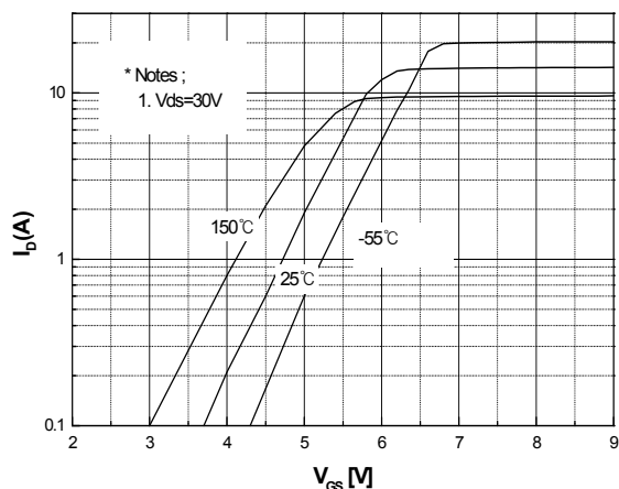
Fig.5 Transfer Characteristics
