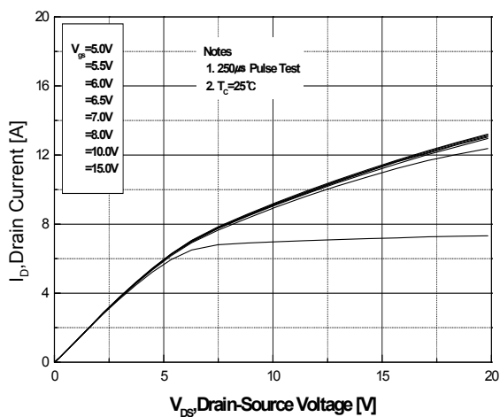
Fig.1 On-Region Characteristics
