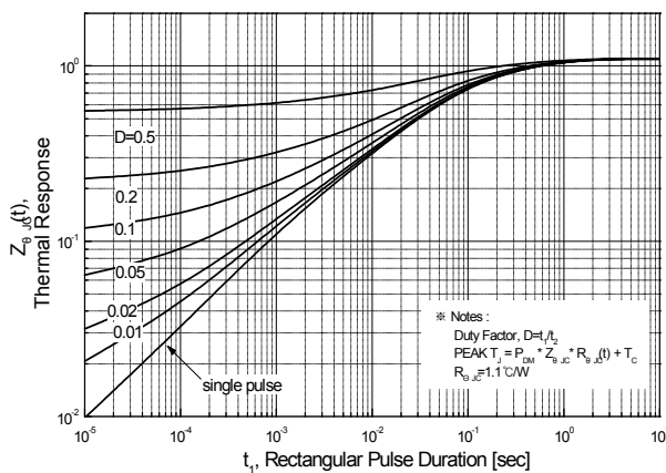
Fig.11 Transient Thermal Response Curve MDP7N50B (TO-220)
