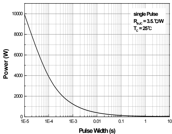
Fig.14 Single Pulse Maximum Power Dissipation – MDF7N50B (TO-220F)
