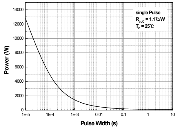
Fig.12 Single Pulse Maximum Power Dissipation – MDP7N50B (TO-220)
