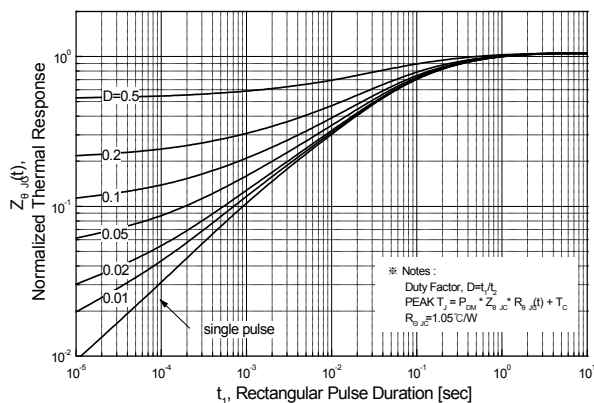
Fig.11 Transient Thermal Response Curve MDP9N50B (TO-220)
