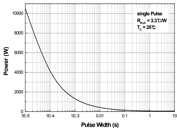
Fig.14 Single Pulse Maximum Power Dissipation – MDF9N50B (TO-220F)
