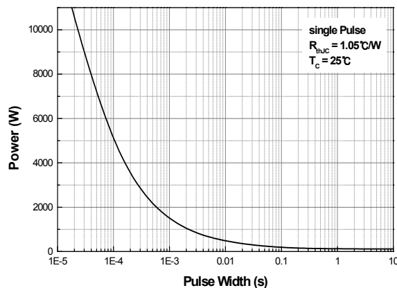
Fig.12 Single Pulse Maximum Power Dissipation – MDP9N50B (TO-220)
