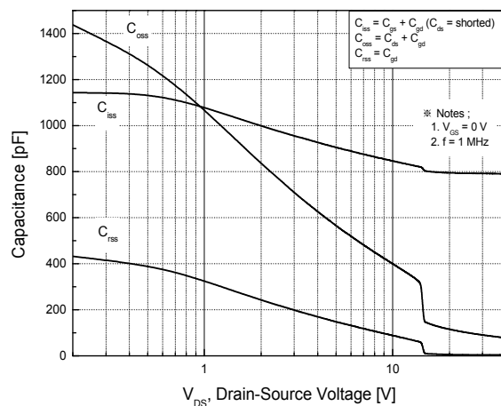
Fig.8 Capacitance Characteristics
