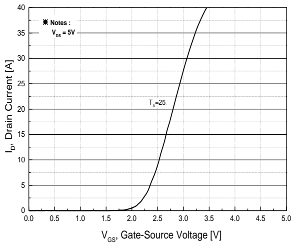
Fig.5 Transfer Characteristics
