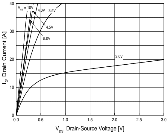
Fig.1 On-Region Characteristics
