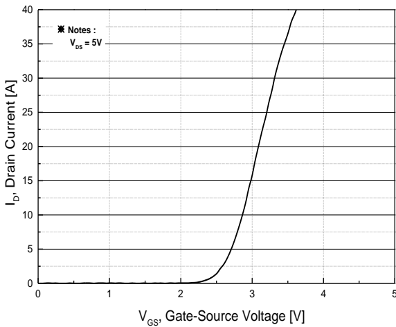
Fig.5 Transfer Characteristics
