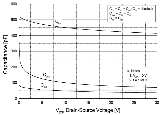
Fig.8 Capacitance Characteristics
