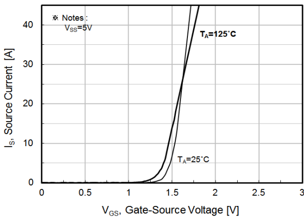
Fig.5 Transfer Characteristics
