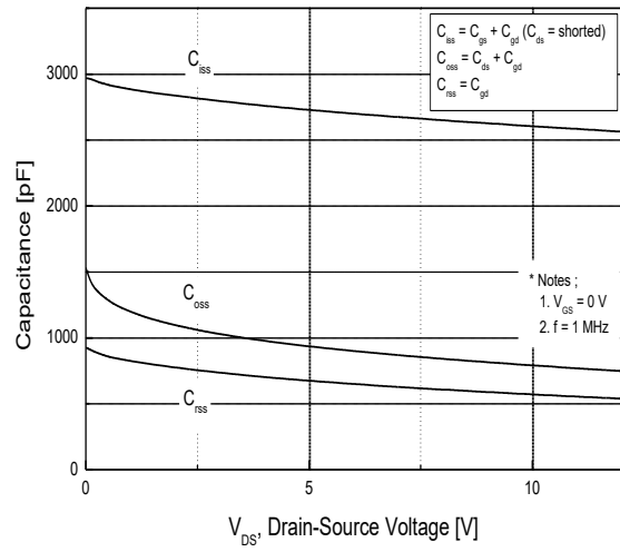
Fig.8 Capacitance Characteristics
