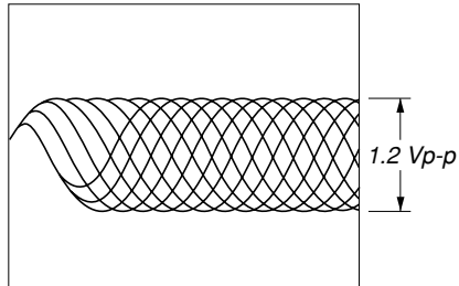
③ IC302 ③⑧ (RF) (PLAY MODE)
