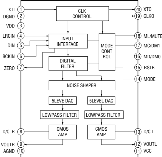
IC202 PCM1717E-ST2
