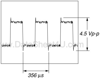
⑤ IC301 ②⑥ (XBCK) (PLAY MODE)
