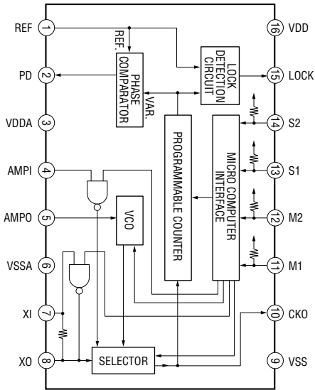
IC200 TC9246F-TP1
