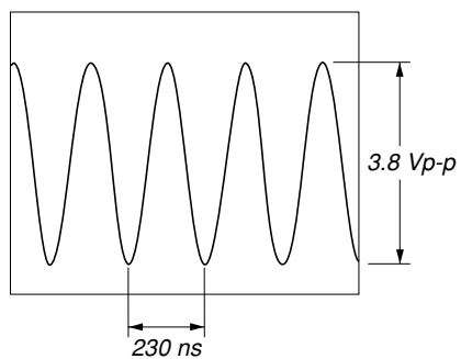
⑨ IC100 ① (XI) (RADIO MODE)
