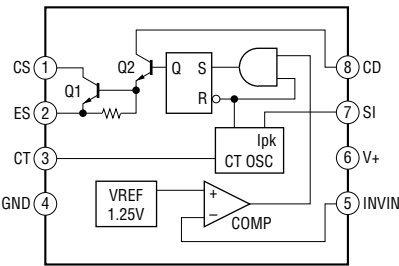
IC250 NJM2360AM (TE2)
