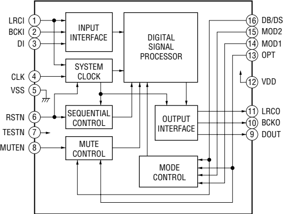
IC201 SM5852FS-E2
