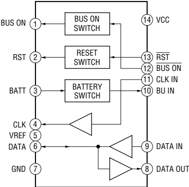
IC600 BA8270F-E2
