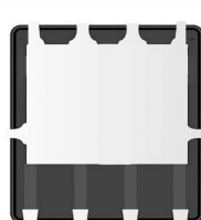
PDFN3X3-8L view
