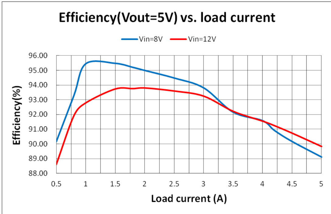
Fig.2 Efficiency1 (Vout=5V)
