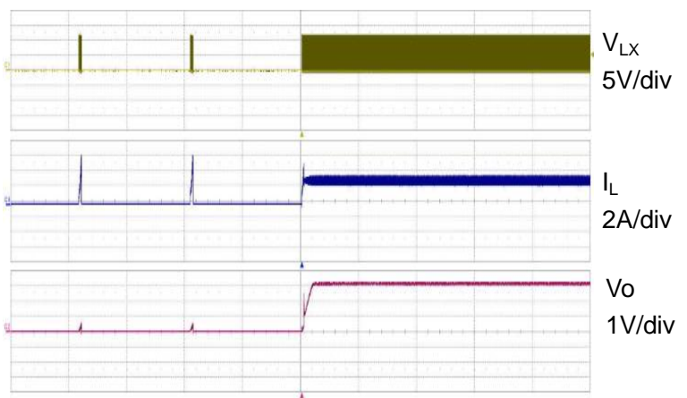
Fig.9 短路恢复 20ms/div
