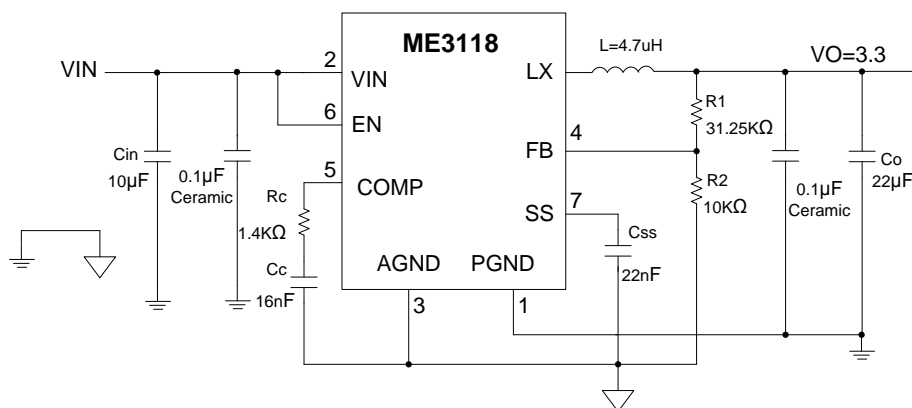
Fig.1 3.3V 3A同步整流降压, Fs = 500 KHz
