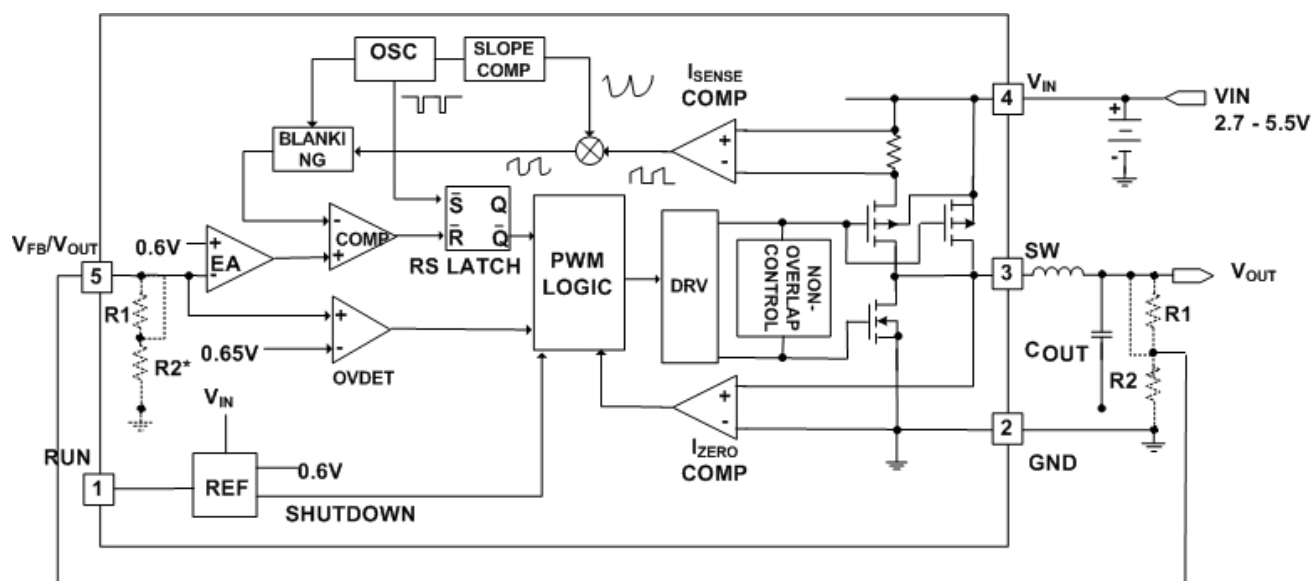
Figure 2. ME3406 Block Diagram
