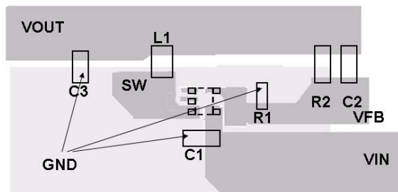
Figure 3. ME3406 Layout Example
