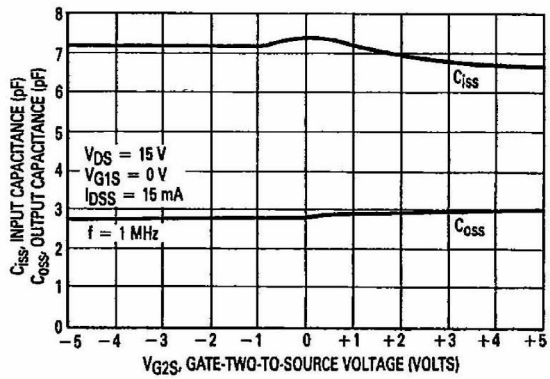
Figure 9. Input and Output Capacitance versus Gate-Two-to-Source Voltage
