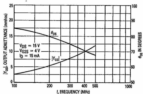
Figure 13. Small-Signal Gate-One Output Admittance versus Frequency
