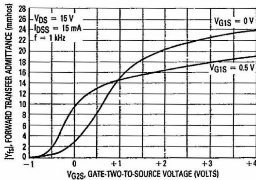
Figure 6. Forward Transfer Admittance versus Gate-Two-to-Source Voltage
