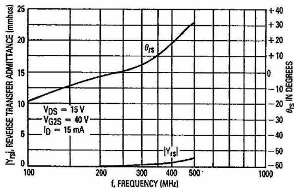
Figure 12. Small-Signal Gate-One Reverse Transfer Admittance versus Frequency
