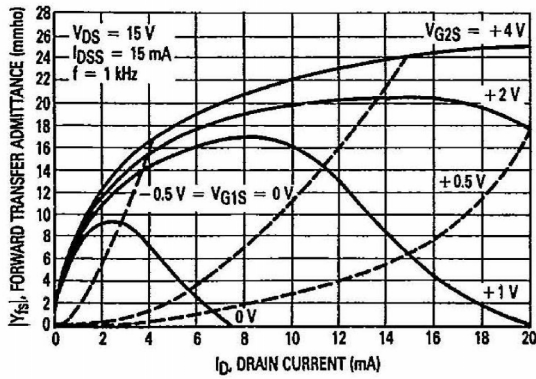
Figure 8. Forward Transfer Admittance versus Drain Current
