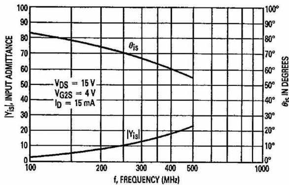
Figure 10. Small-Signal Gate-One Input Admittance versus Frequency
