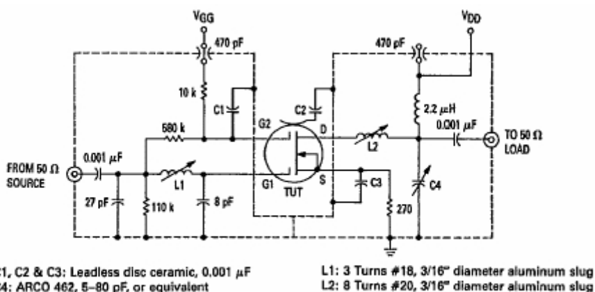
Figure 1. 200 MHz Power Gain, Gain Control Voltage, and Noise Figure Test Circuit for MFE211
