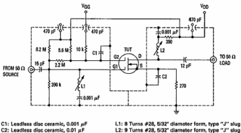
Figure 2. 45 MHz Power Gain and Noise Figure Test Circuit for MFE211
