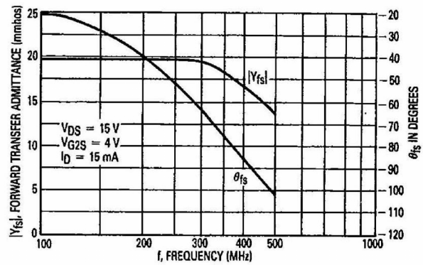
Figure 11. Small-Signal Forward Transfer Admittance versus Frequency
