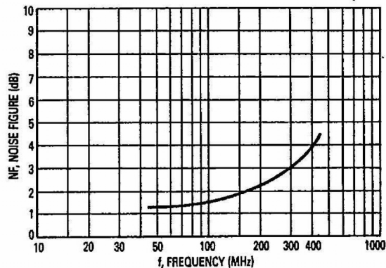
Figure 17. Optimum Spot Noise Figure versus Frequency
