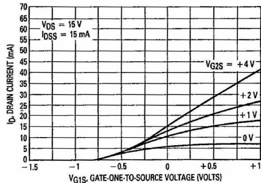
Figure 5. Drain Current versus Gate-One-to-Source Voltage
