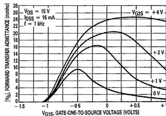
Figure 7. Forward Transfer Admittance versus Gate-One-to-Source Voltage
