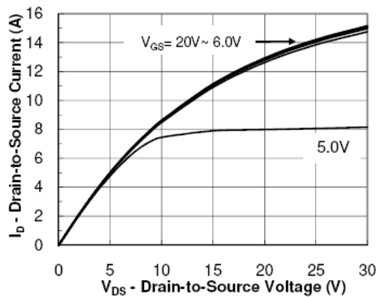
Figure1.Output Characteristic
