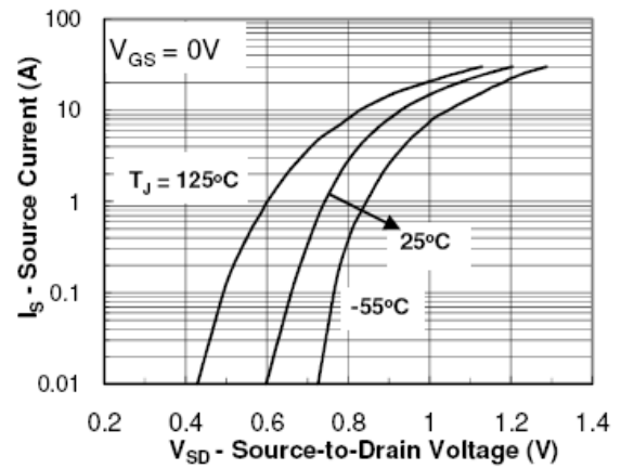
Figure8.Source-Drain Diode
