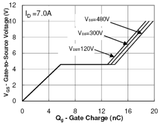
Figure7.Gate Charge Waveform
