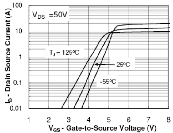
Figure2.Transfer Characteristic
