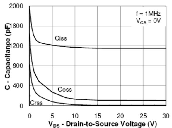
Figure6.Capacitance
