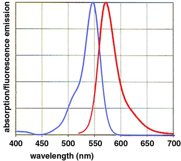
Figure above: Absorption and fluorescence emission spectra of MFP555 dye in ethanol (molar absorbance: 100.000 M^{-1}cm^{-1} ). Absorption and emission maximum shift to 560/585 nm by measuring MFP555 goat anti-mouse IgG antibody in PBS buffer, pH 7.2.
