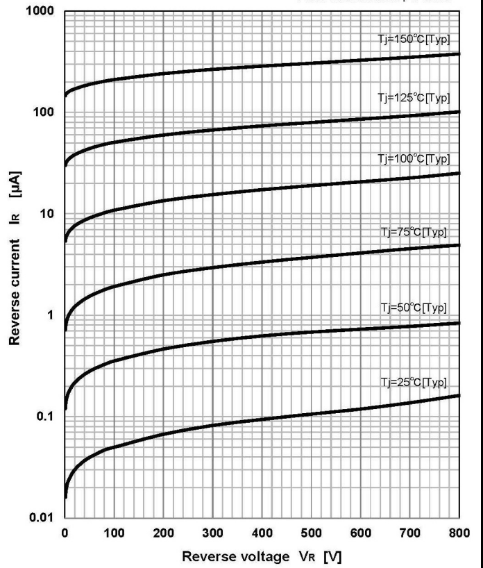
Reverse current
