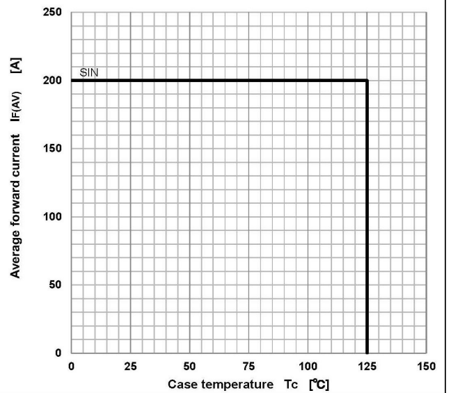
Derating curve
