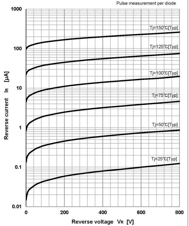
Reverse current
