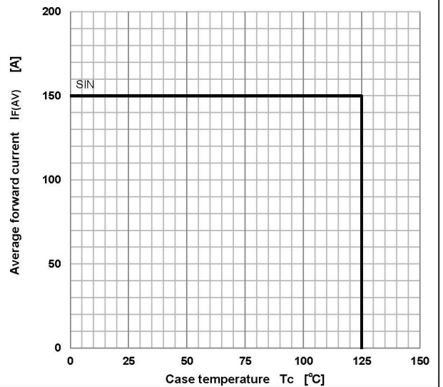
Derating curve
