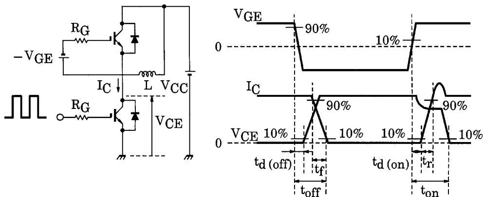
Note 1: Switching time test circuit & timing chert
