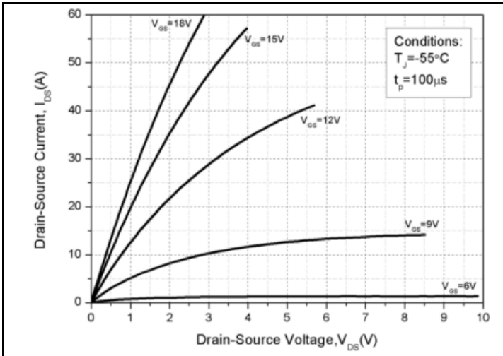
Output Characteristics T_J = -55^\circ\text{C}
