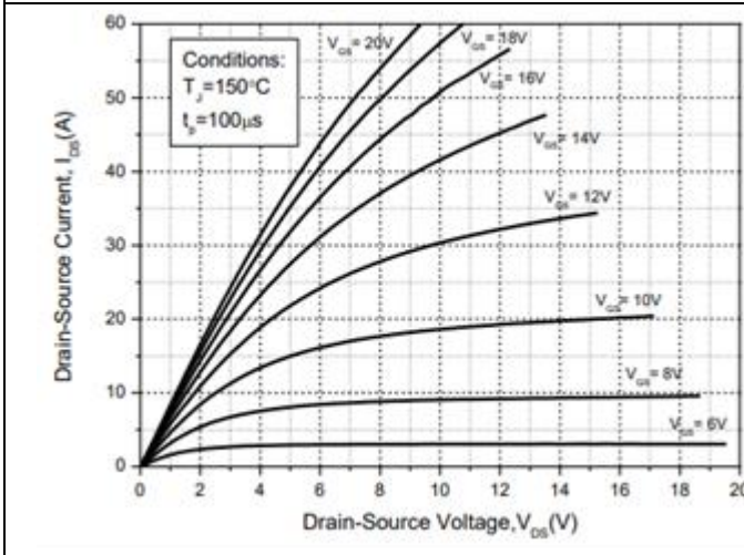
Output Characteristics T_J = 150^\circ\text{C}
