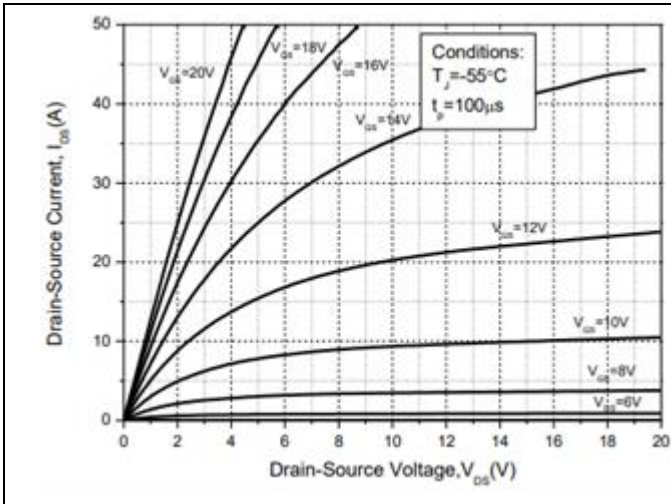
Output Characteristics T_J = -55^\circ\text{C}
