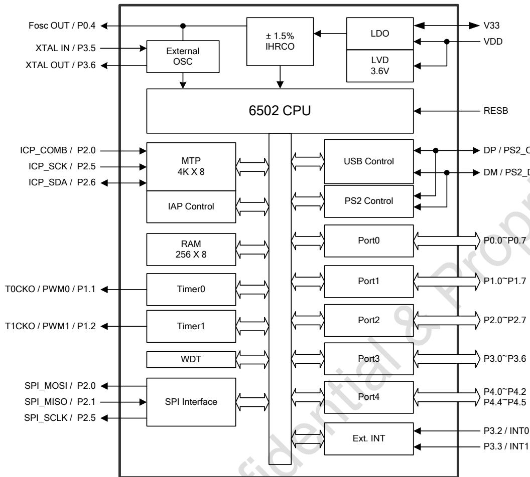
Figure 3-1 Block Diagram
