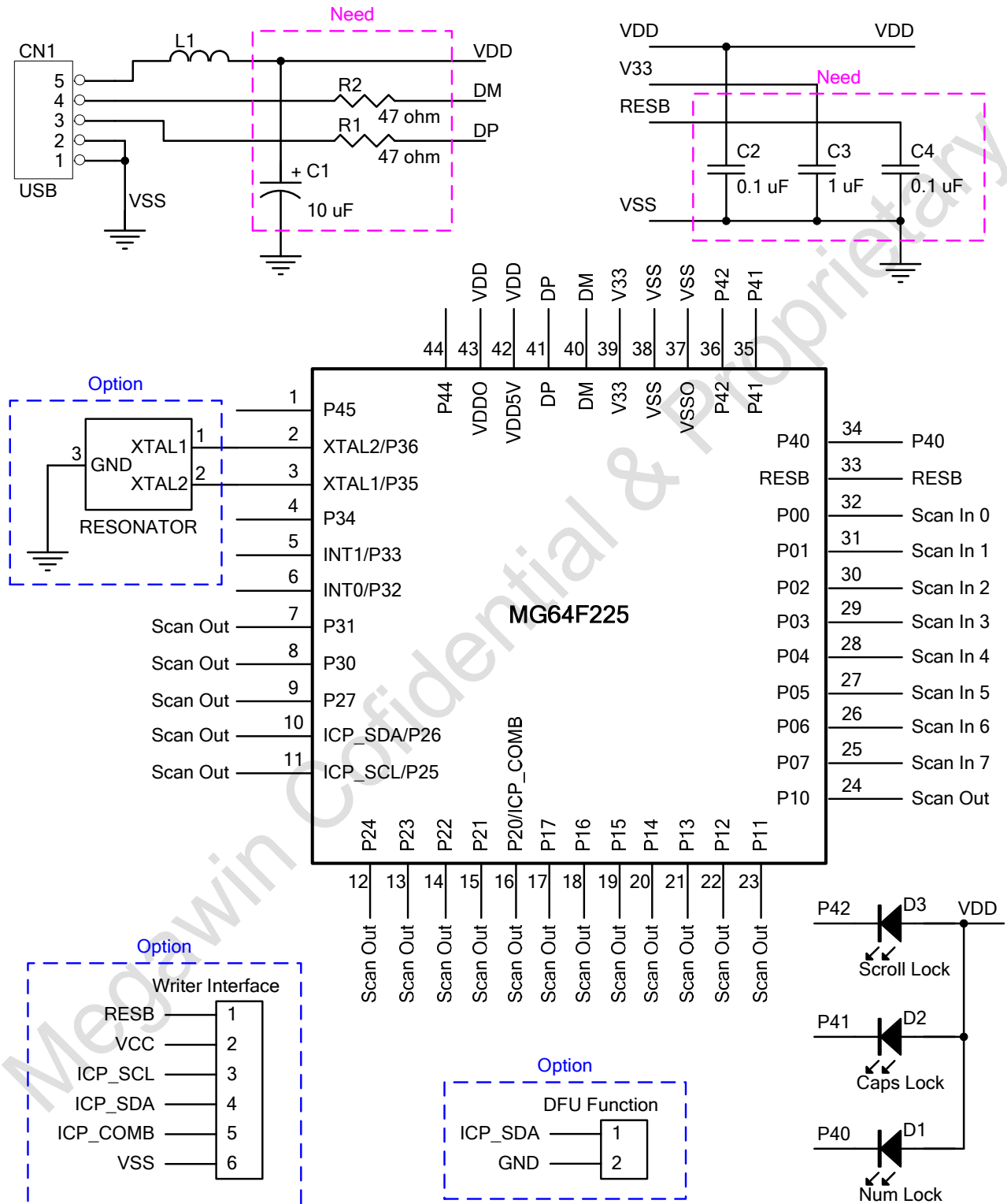
Figure 18-1 Application Circuit - Keyboard
