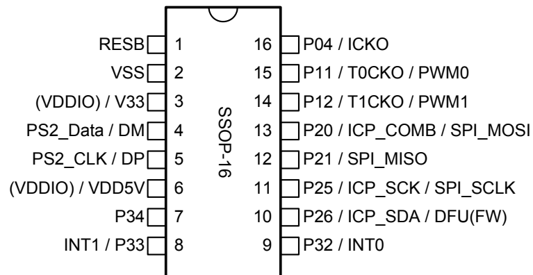
Figure 4-2 Package SSOP16
