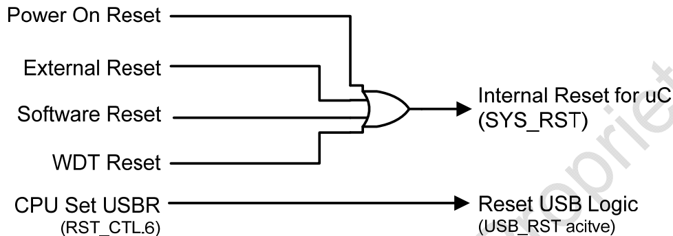
Figure 11-1 Reset Source
