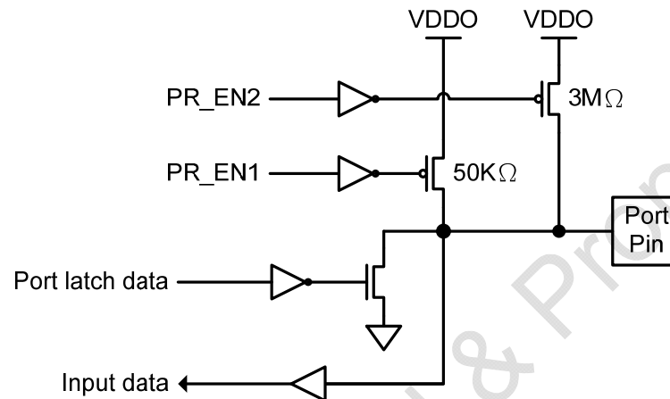
Figure 7-1 GPIO Diagram
