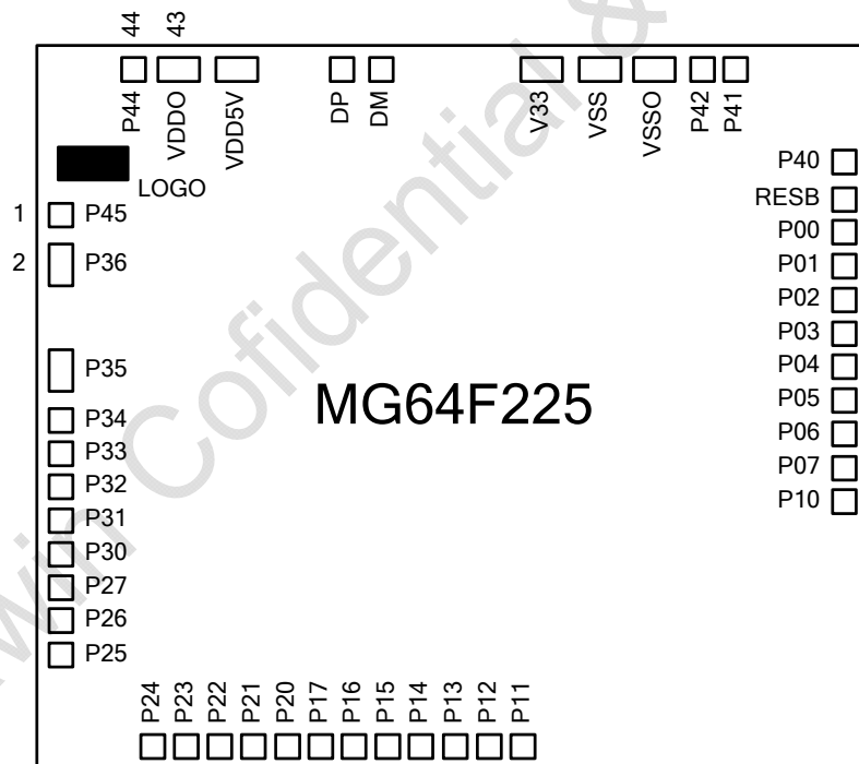
Figure 4-3 Dice
