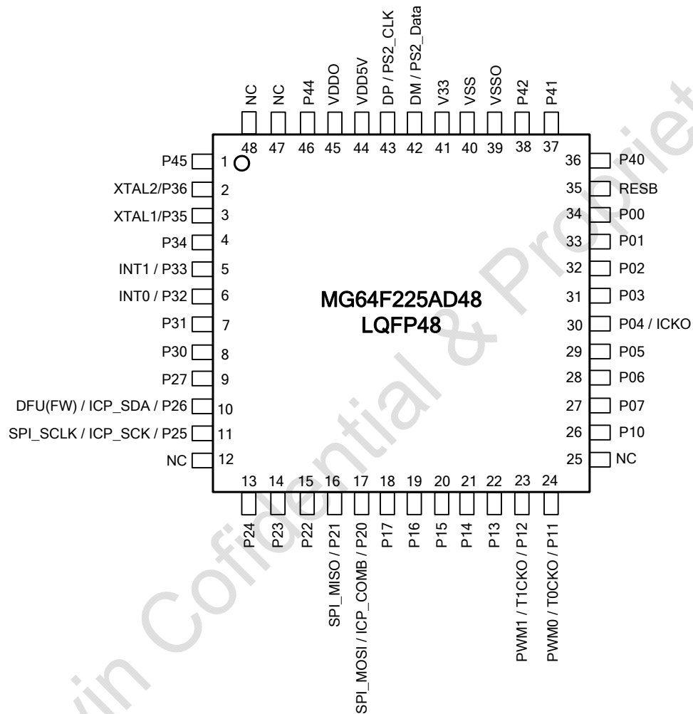
Figure 4-1 Package LQFP48
