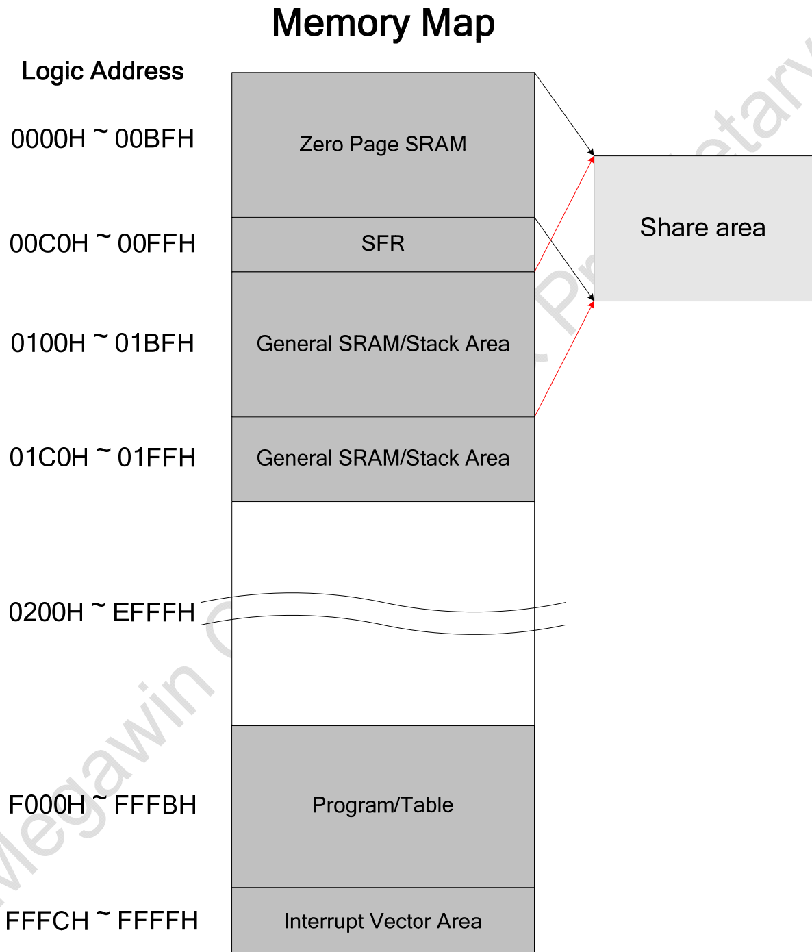
Figure 6-1 Memory Map
