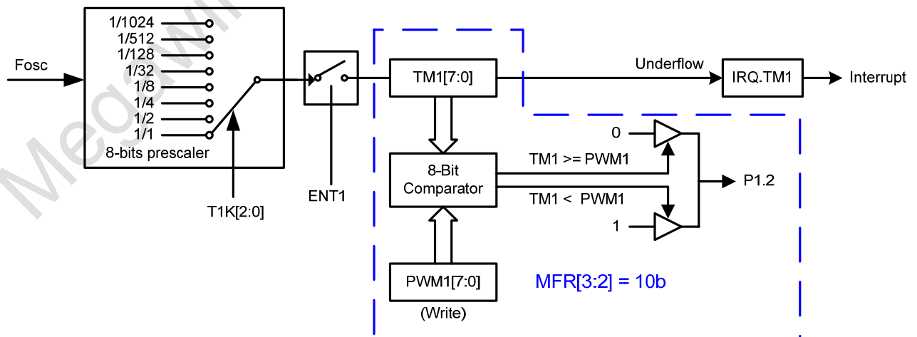
Figure 9-4 Timer1 / PWM1 Structure – PWM Mode
