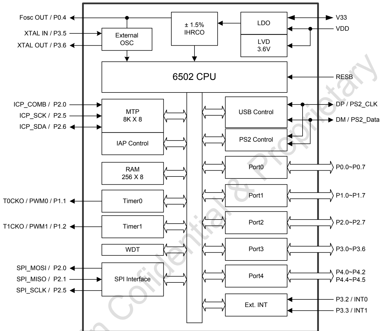
Figure 3-1 Block Diagram
