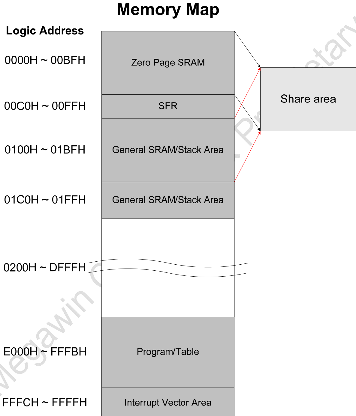
Figure 6-1 Memory Map
