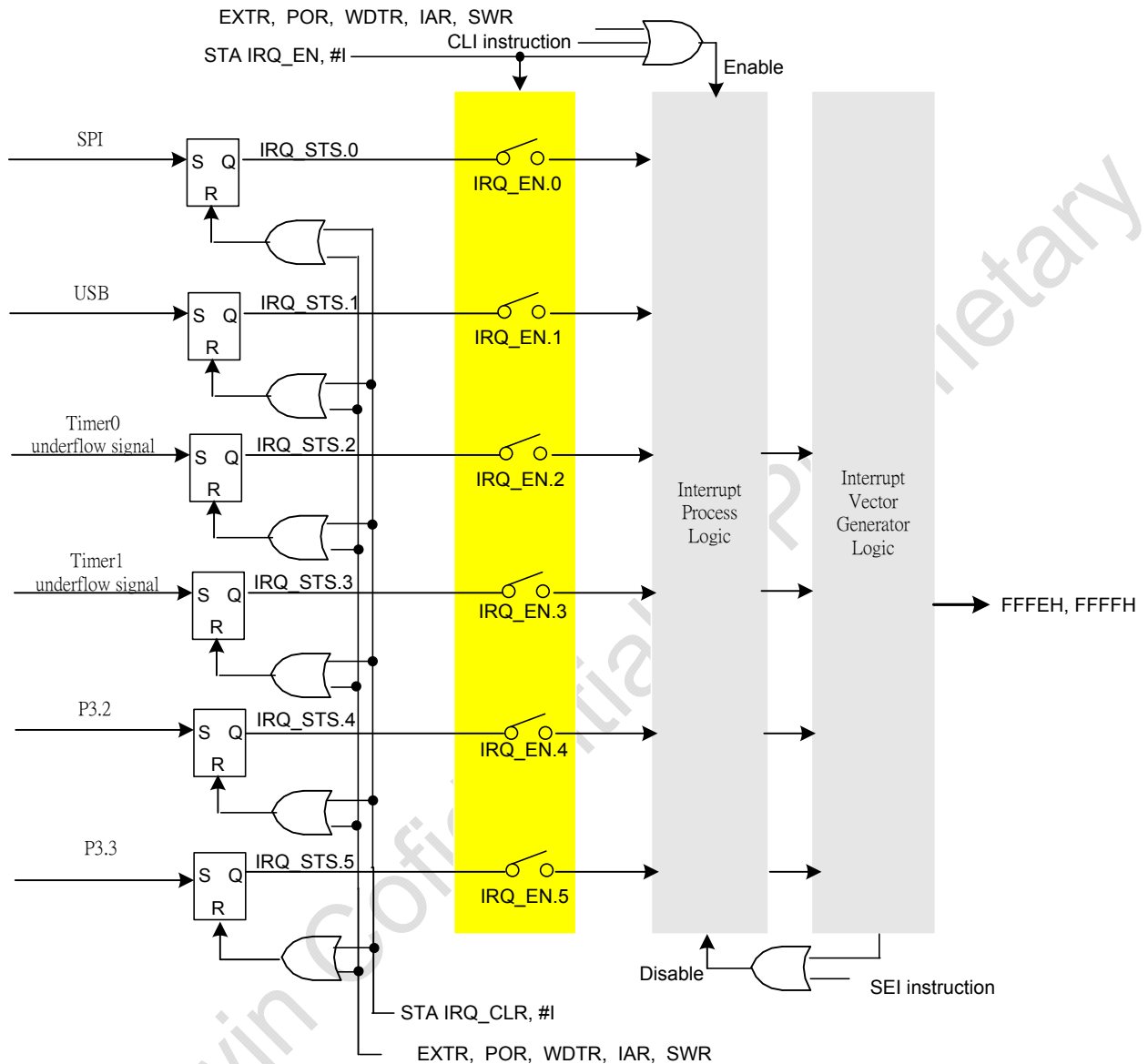
Figure 8-1 Interrupt Diagram
