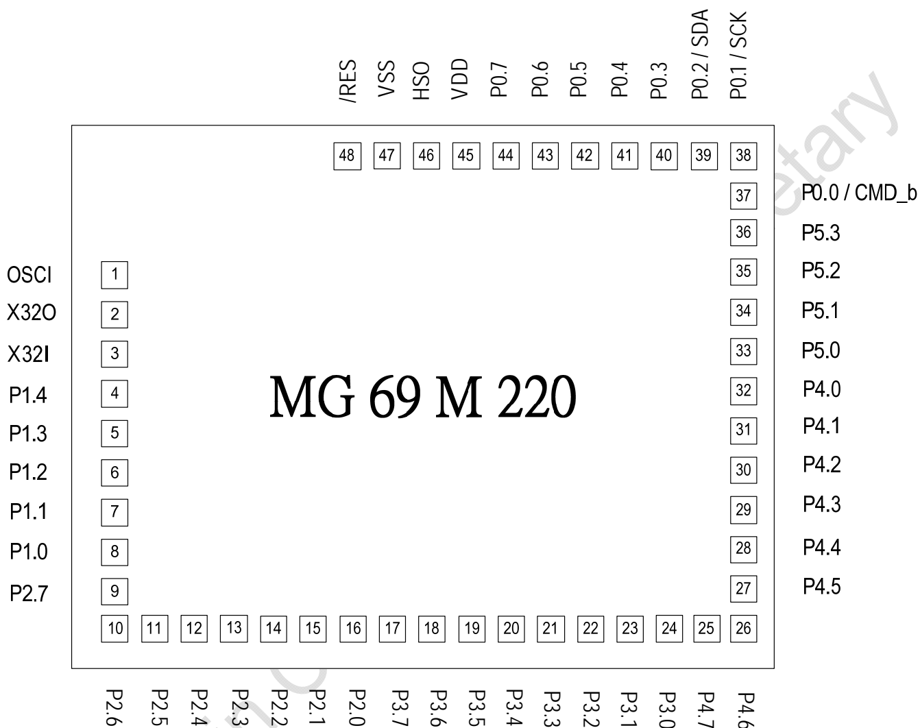
Figure 3-1 Pad Assignment
