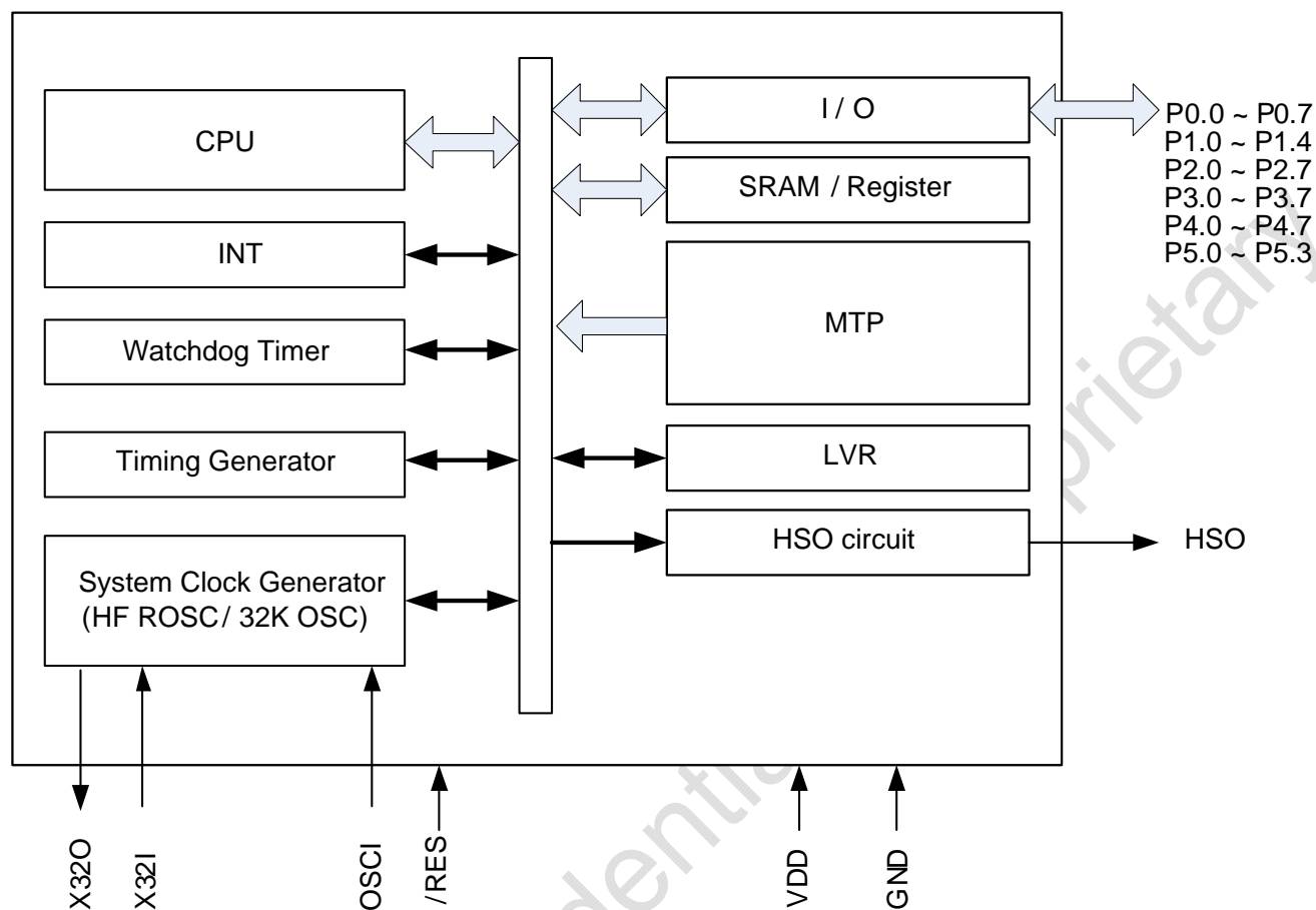
Figure 4-1 Block Diagram
