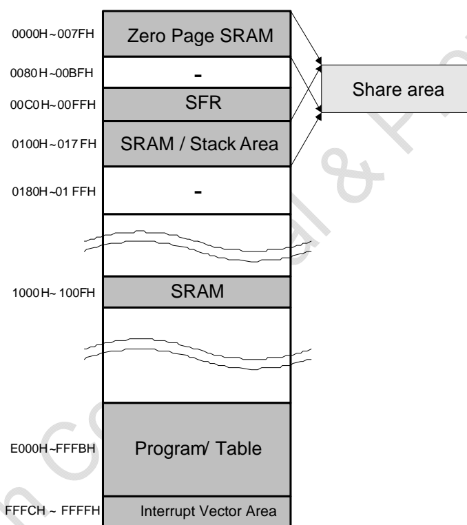
Figure 6-1 Memory Map
