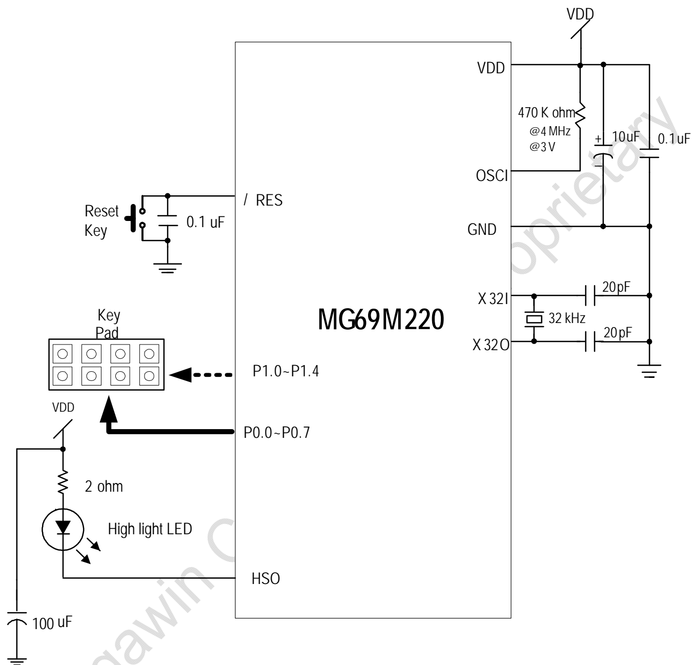
Figure 14-1 Application Circuit – Key Pad Controller
