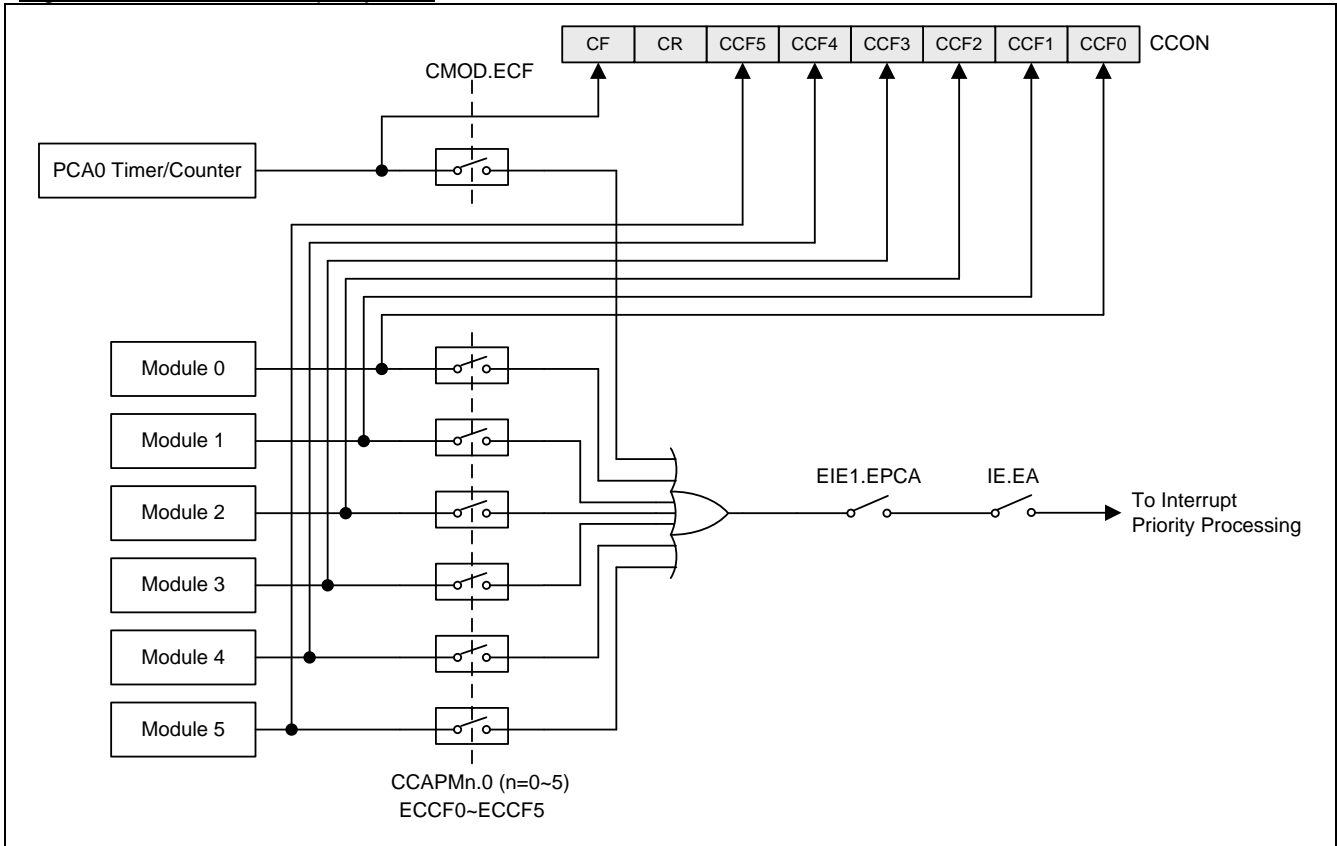
Figure 16–3. PCA Interrupt System
