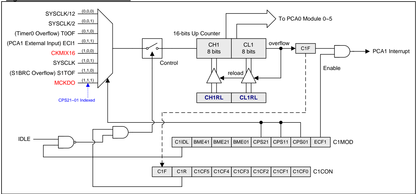
Figure 17-2. PCA1 Timer/Counter
