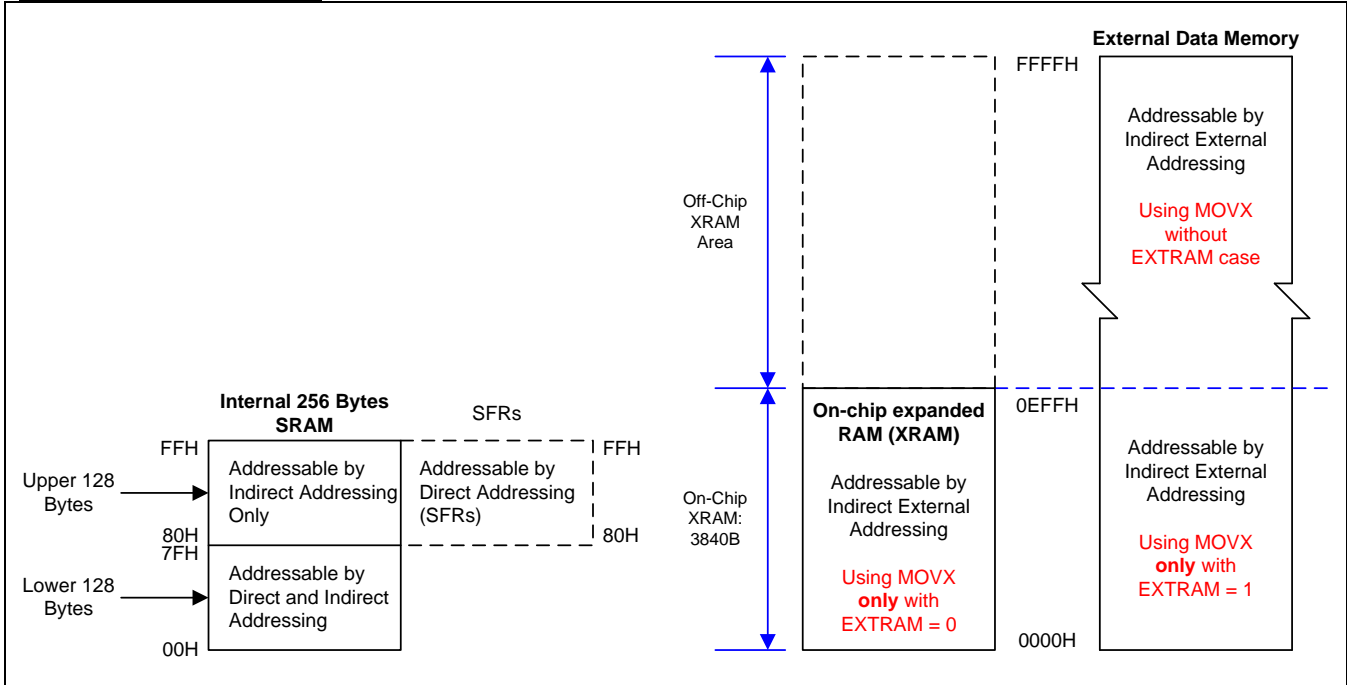
Figure 6–2. Data Memory
