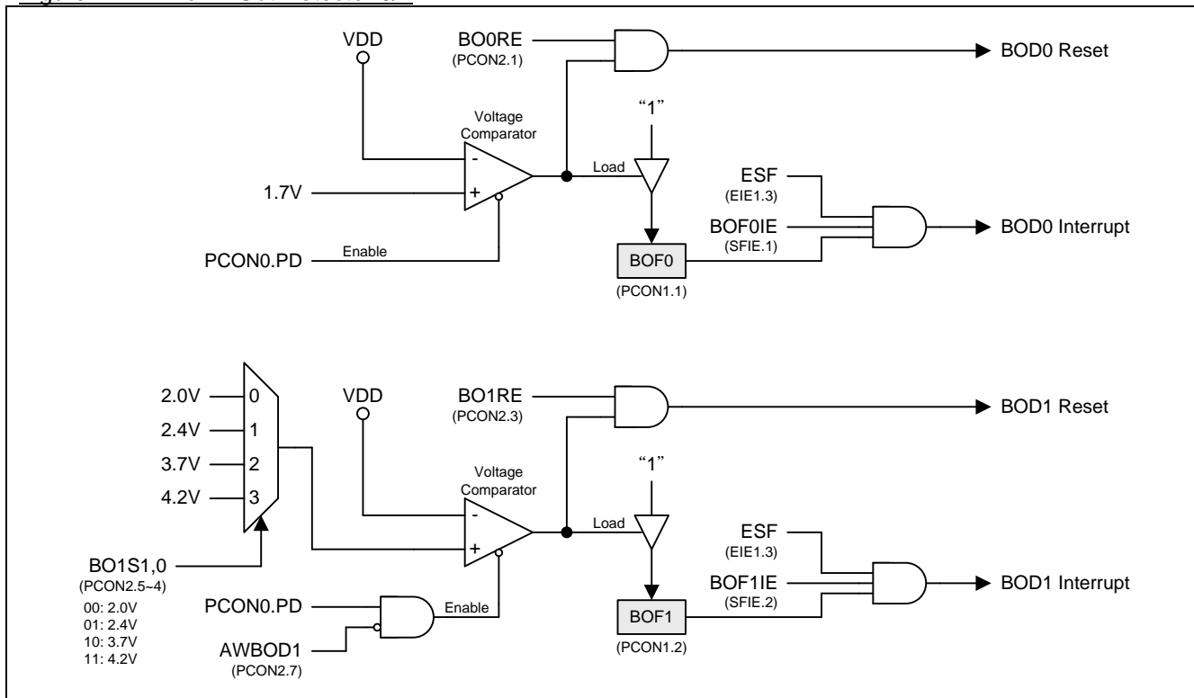
Figure 12–1. Brown-Out Detector 0/1
