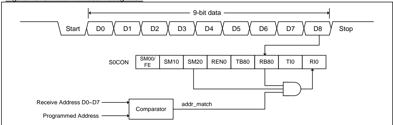
Figure 18–9. Auto-Address Recognition
