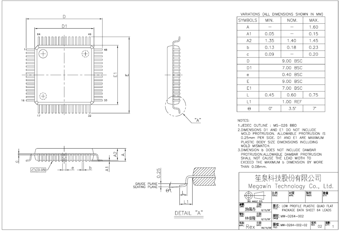
Figure 36-1 LQFP-64 (7mm X 7mm )
