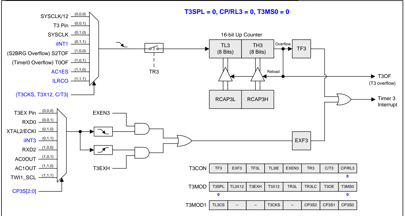
Figure 15–24. Timer 3 Mode 0 Structure (Auto-Reload and External Interrupt Mode)
