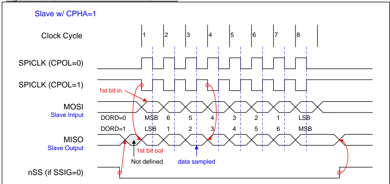
Figure 22–6. Slave Transfer Format with CPHA=1
