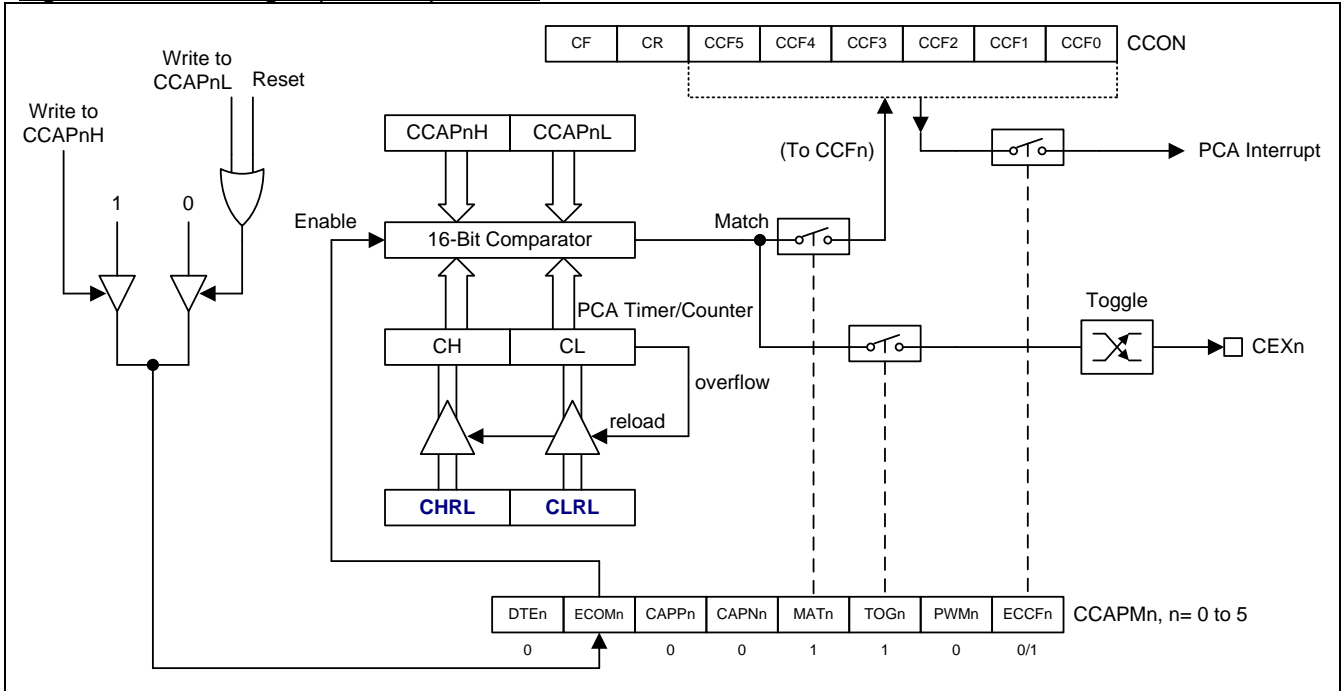
Figure 16–8. PCA High Speed Output Mode
