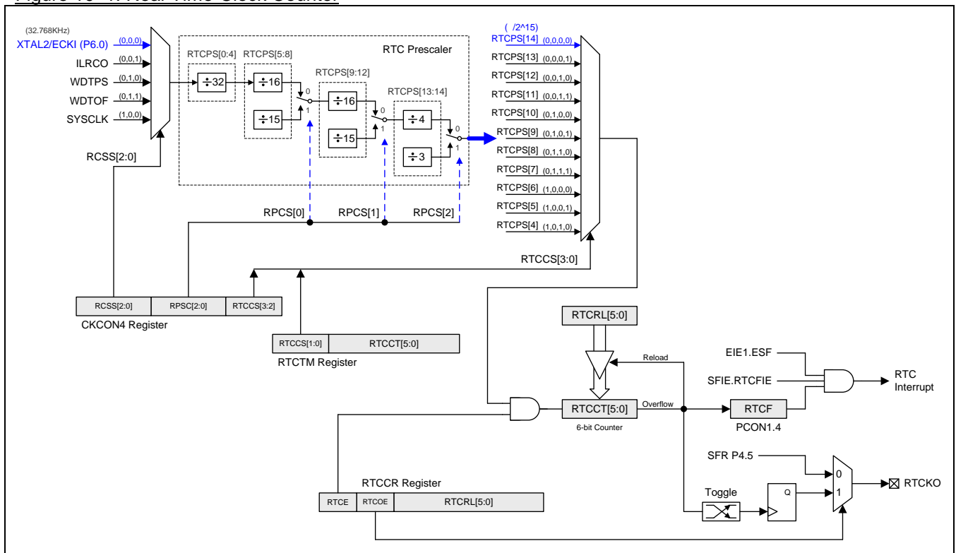
Figure 10–1. Real-Time-Clock Counter
