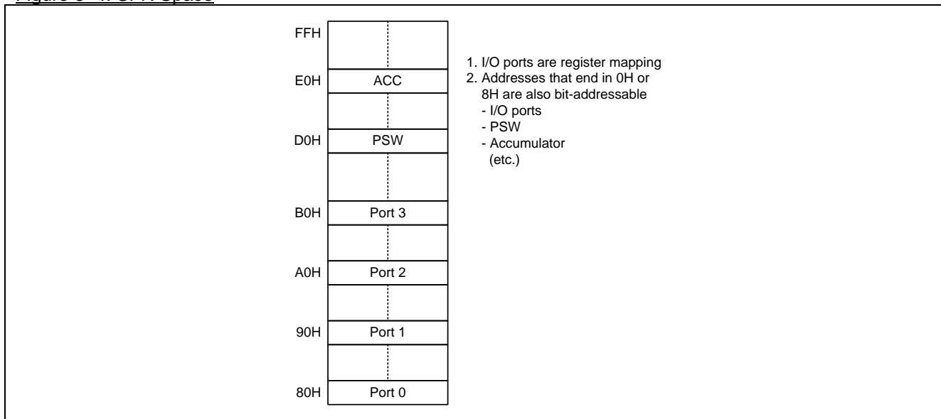
Figure 6–4. SFR Space
