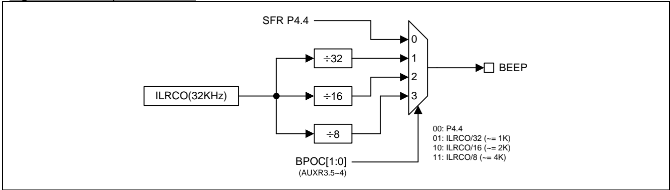
Figure 25–1. Beeper Generator
