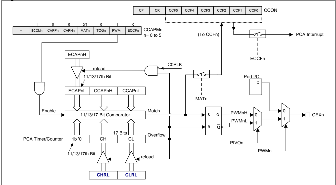
Figure 16–11. PCA Enhance PWM for Buffer Mode
