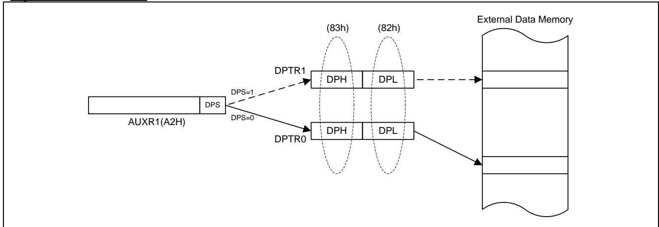
Figure 7-1. Dual DPTR
