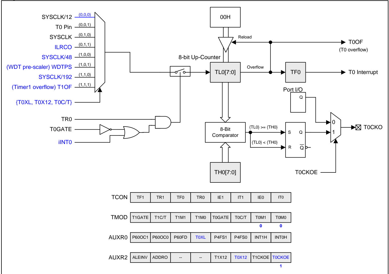
Figure 15–1. Timer 0 Mode 0 Structure
