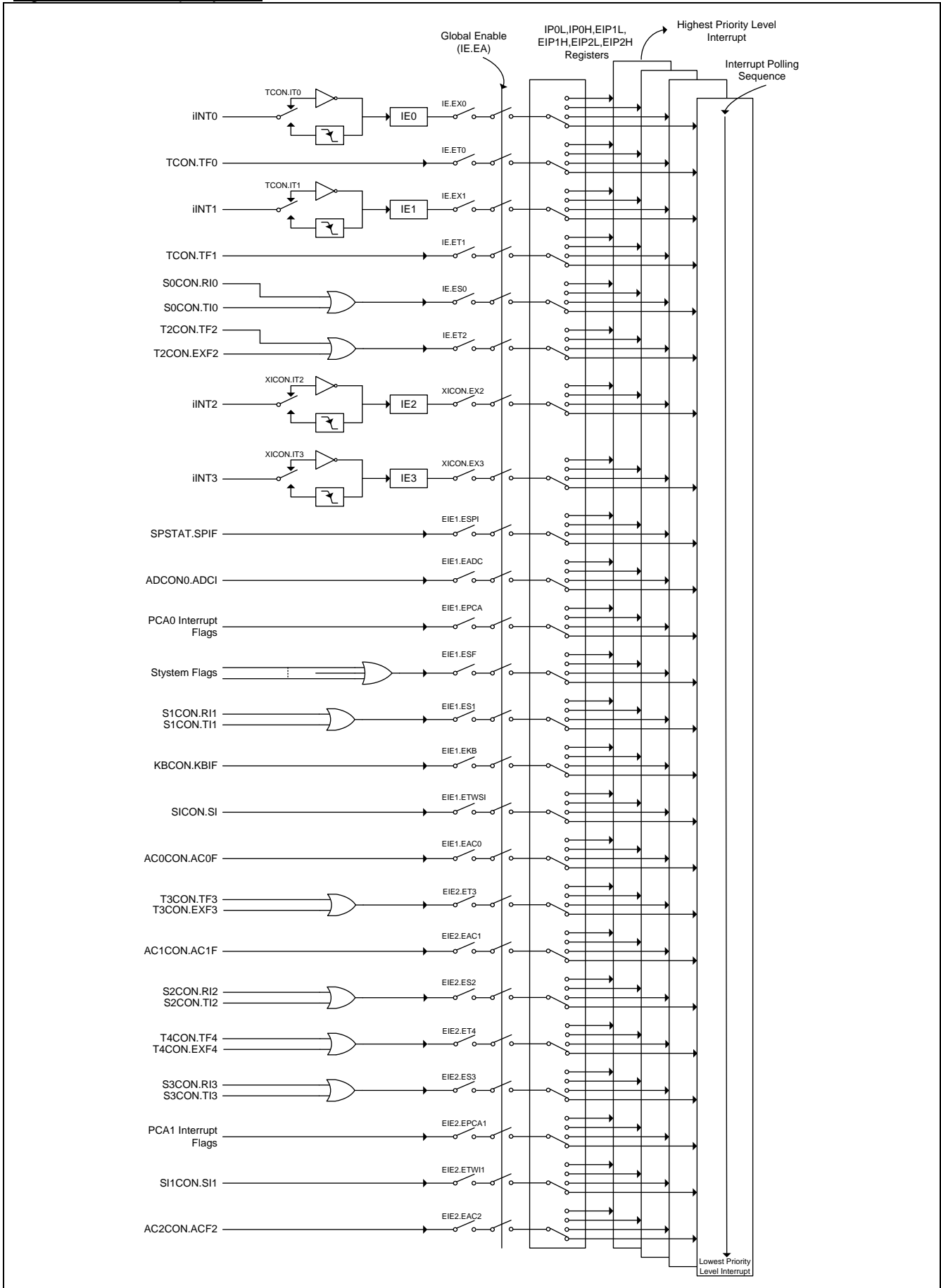
Figure 14–1. Interrupt System
