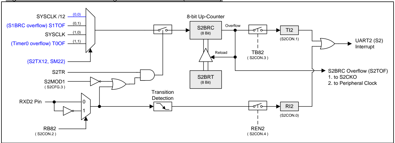
Figure 20–1. Timer Mode Configuration for S2BRG (S2TME=1)
