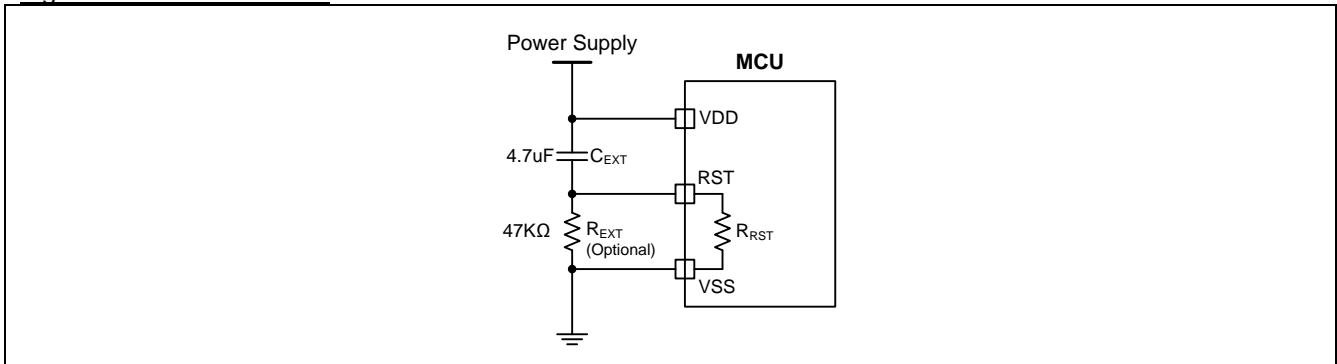
Figure 33–2. Reset Circuit
