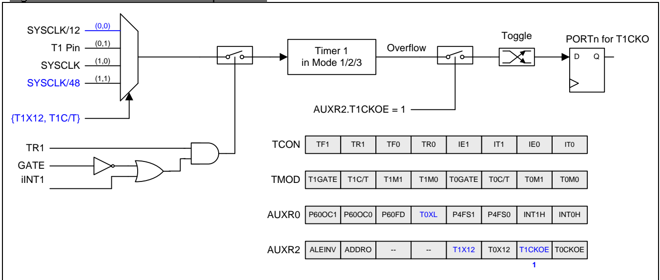
Figure 15–11. Timer 1 in Clock Output Mode
