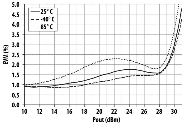
Figure 7. Over-temperature EVM vs Output Power at 728 MHz
