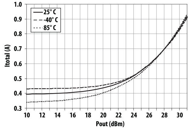
Figure 8. Over-temperature I_{dd\_total} vs Output Power at 728 MHz
