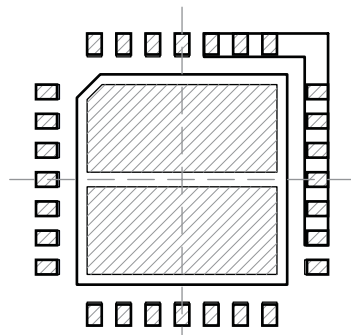
COMBINED PCB LAND PATTERN AND STENCIL OUTLINE
