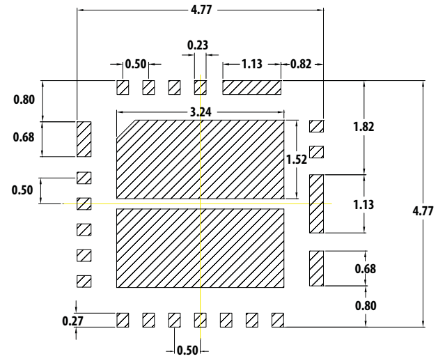
Stencil Opening
