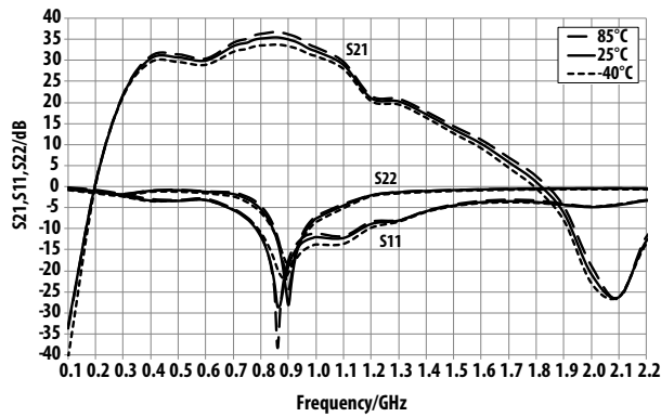
Figure 6. Small-signal performance Over-temperature V_{dd}=V_{ddBias}=5.0 V operating voltage
