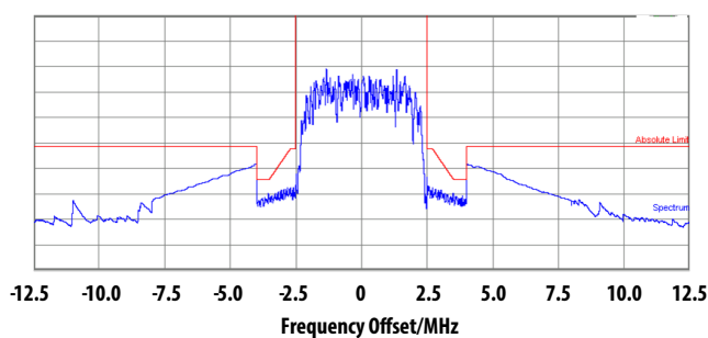
Figure 25. SEM at P_{out}=28 dBm @ 957.6 MHz
