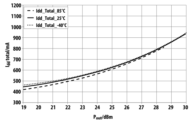
Figure 15. Over-temperature I_{dd\_Total} vs. P_{out} @ 940 MHz V_{dd}=V_{ddBias}=5.5 V operating voltage
