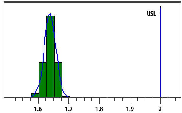
Figure 5. NF Distribution
