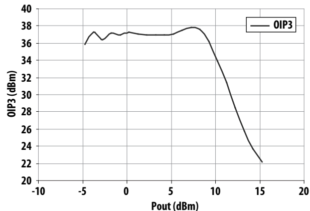
Figure 23. OIP3 vs Output Power at 1900MHz
