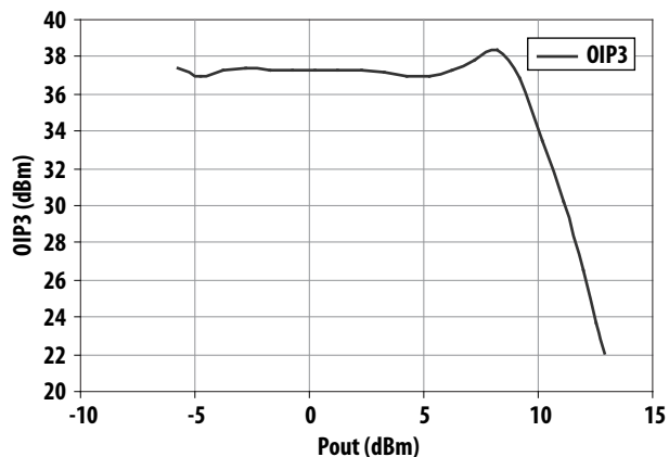
Figure 32. OIP3 vs Output Power at 2400MHz
