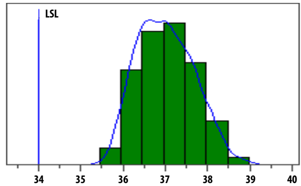
Figure 3. OIP3 Distribution
