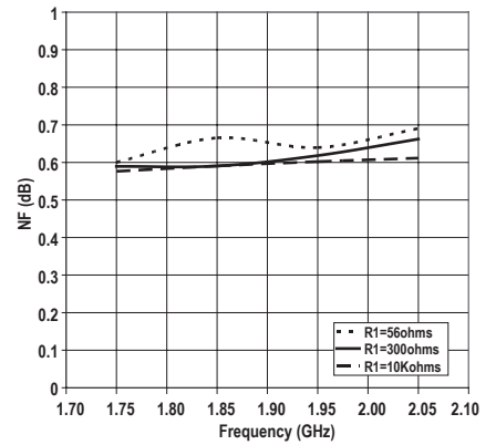
Figure 18. NF vs Frequency and R1
