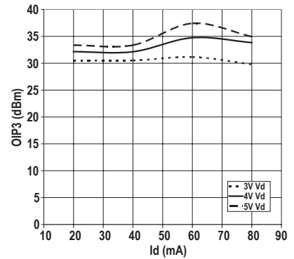
Figure 9. OIP3 Vs I_d and V_d
