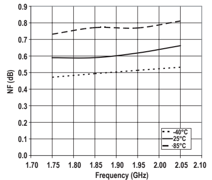
Figure 12. NF Vs Frequency and Temperature
