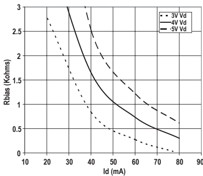
Figure 10. R_{bias} Vs I_d and V_d
