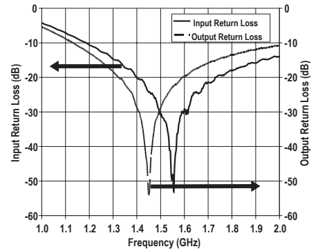
Figure 24. Input and output Return Loss vs Frequency
