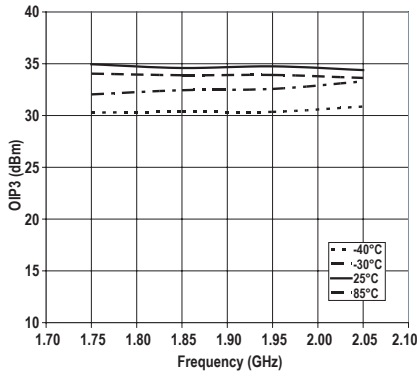
Figure 13. OIP3 vs Frequency and Temperature
