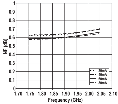
Figure 5. NF Vs Frequency and I_d
