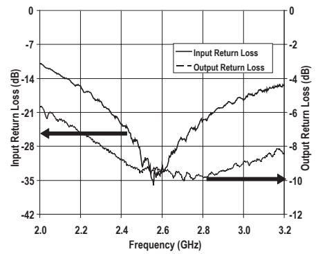
Figure 27. Input and output Return Loss vs Frequency
