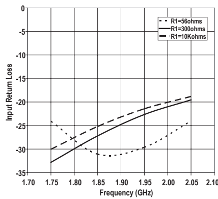
Figure 20. Input Return Loss vs Frequency and R1
