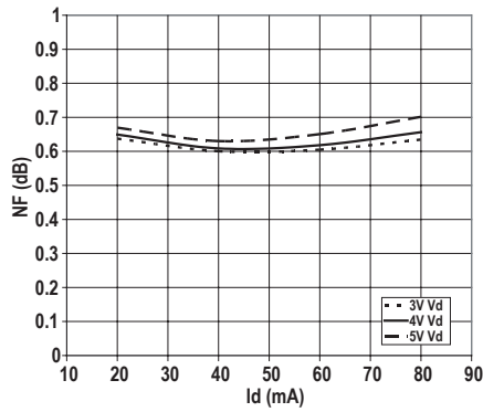
Figure 8. NF Vs I_d and V_d
