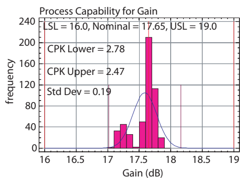
Figure 1. Gain distribution at 60mA
