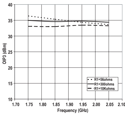
Figure 19. OIP3 vs Frequency and R1
