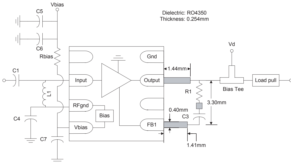
Figure 30. Test setup for load pull data
