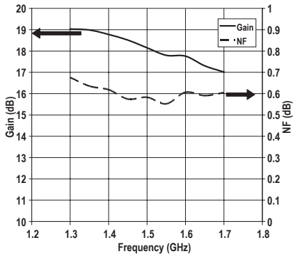
Figure 22. Gain and NF Vs Frequency
