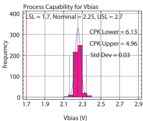
Figure 3. Vbias distribution at 60mA
