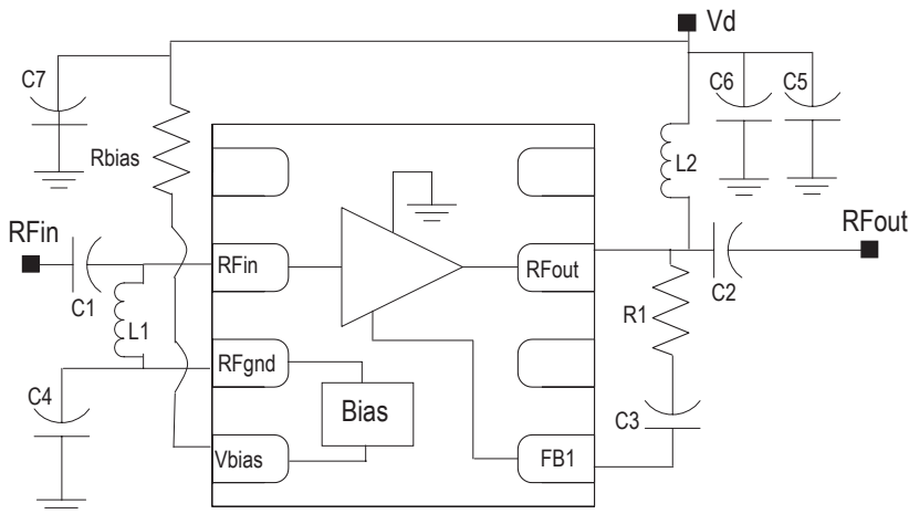
Figure 29. Demo Board Schematic. This demo board is used for the measurement.
