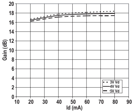
Figure 7. Gain Vs I_d and V_d
