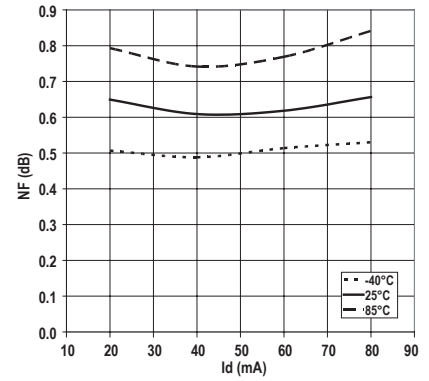
Figure 15. NF vs Id and Temperature
