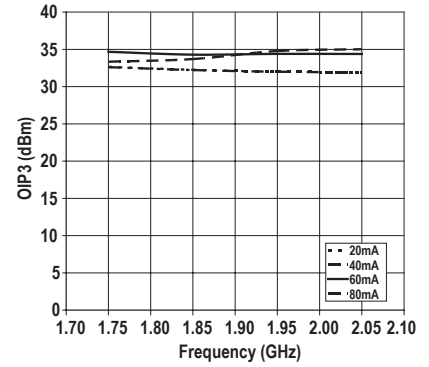
Figure 6. OIP3 Vs Frequency and I_d
