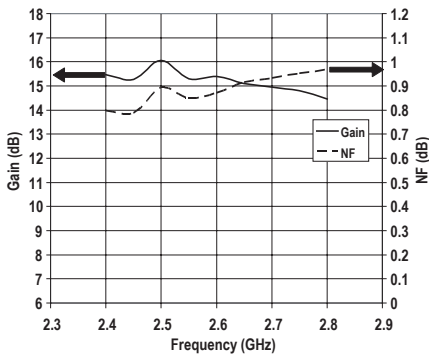
Figure 25. Gain and NF vs Frequency
