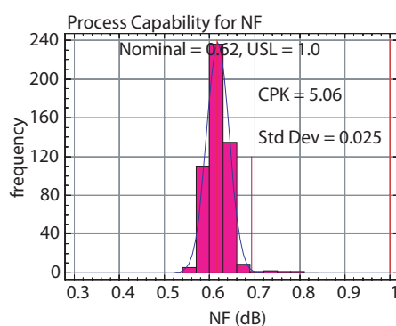
Figure 2. NF distribution at 60mA
