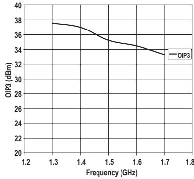
Figure 23. OIP3 vs Frequency
