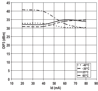
Figure 16. OIP3 vs Id and Temperature
