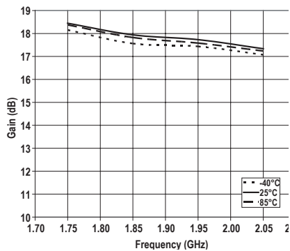
Figure 11. Gain Vs Frequency and Temperature
