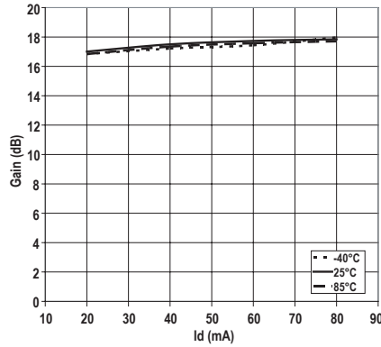
Figure 14. Gain vs Id and Temperature
