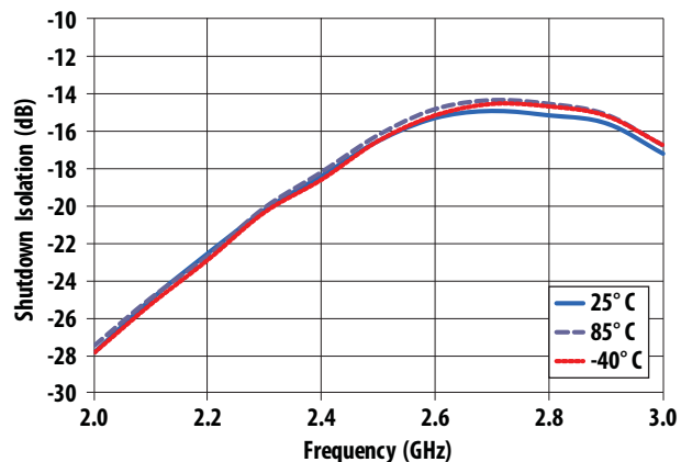
Figure 37. Shutdown Mode Isolation vs Frequency vs Temperature
