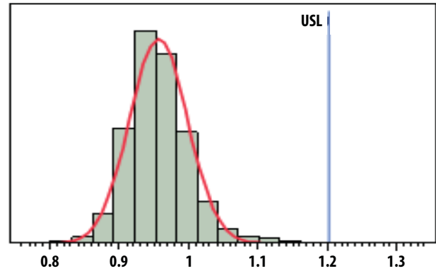
Figure 2. NF @ 2.4 GHz, V_{dd} 3\text{ V} ; V_{bias} 1.8\text{ V} Nominal = 0.95 dB, USL = 1.2 dB
