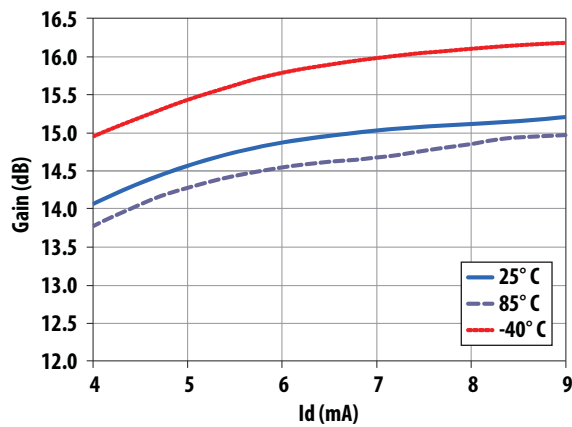
Figure 26. LNA Mode Gain vs I_d vs Temperature
