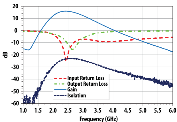
Figure 23. LNA Mode Gain, Input Return Loss, Output Return Loss, Isolation vs Frequency
