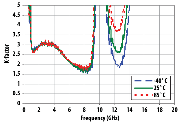
Figure 12. K-factor vs Frequency vs Temperature
