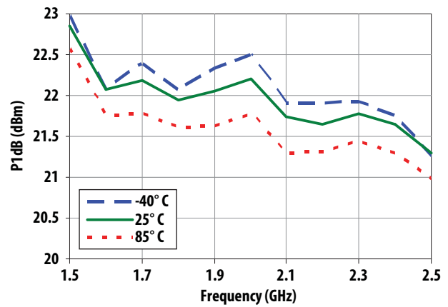
Figure 10. OP1dB vs Frequency vs Temperature
