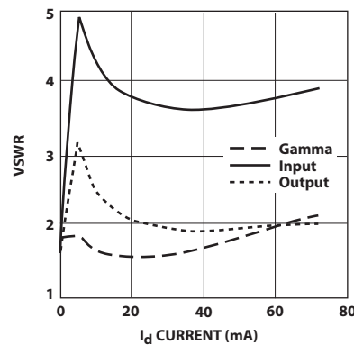
Figure 19. Input and Output VSWR and VSWR of |opt| vs. Current.
