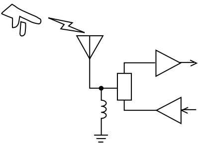
Figure 17. In-circuit ESD Protection.
