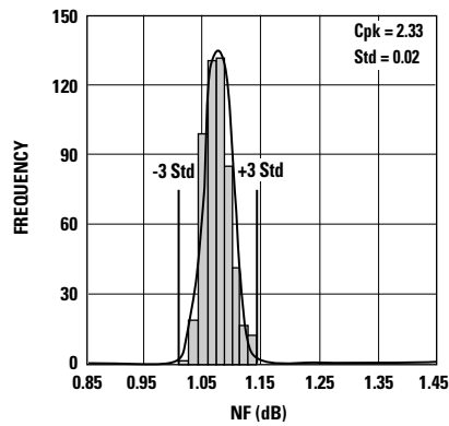
Figure 3. NF @ 2 GHz, 3V, 10 mA. LSL = 0.85, Nominal = 1.08, USL = 1.45
