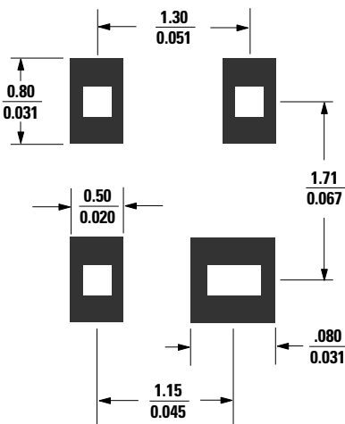
Figure 12. PCB Pad Print for SOT-343 Package (mm/inches).
