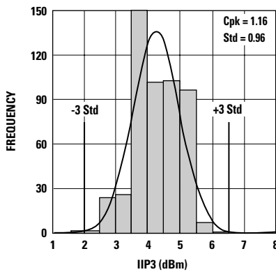
Figure 2. IIP3 @ 2 GHz, 3V, 10 mA. LSL = 1.0, Nominal = 4.3, USL = 8.0
