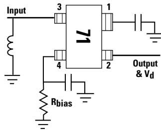
Figure 6. Source Resistor Bias Method.
