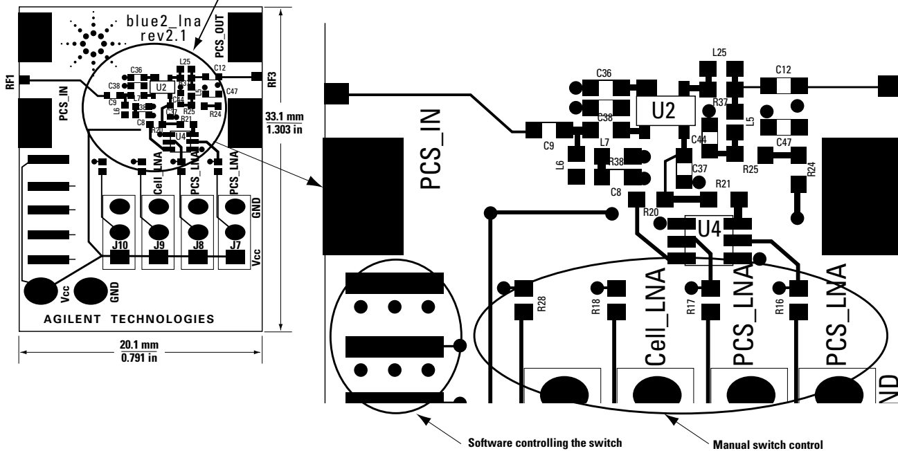
Figure 25. Small Size Amplifier Board with Components for Handset Focussed Designers.
