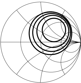
Figure 19. Noise Circles F = 1900 MHz, Step Size: 0.2 dB.
