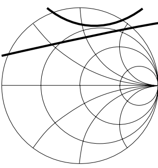
Figure 21. Load and Source Stability Circles.
