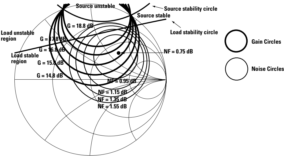
Figure 18. Gain, Noise and Stability Circles.
