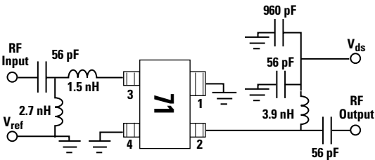
Figure 4. MGA-71543 Production Test Circuit.
