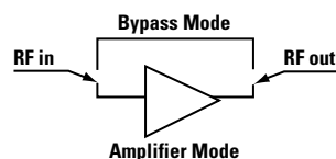
Figure 2. Simplified Schematic.
