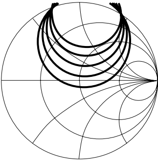
Figure 20. Gain Circle F = 1900 MHz, Step Size: 1.0 dB.
