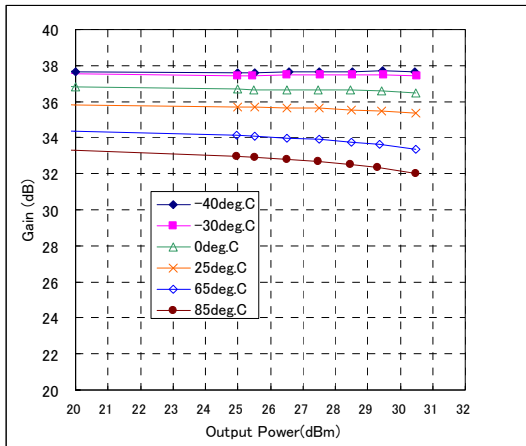
Gain vs. Output Power
