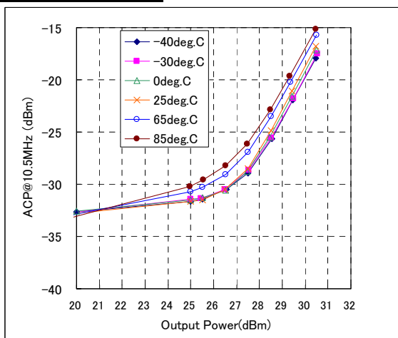
ACP Characteristics
