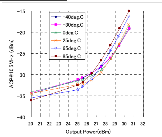
ACP Characteristics
