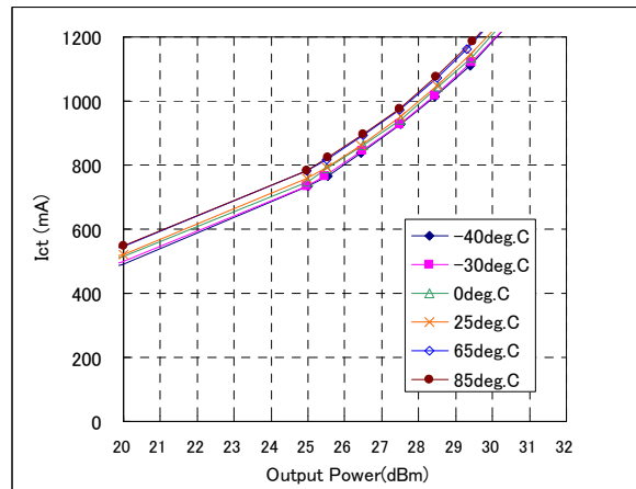
Operating Current vs. Output Power
