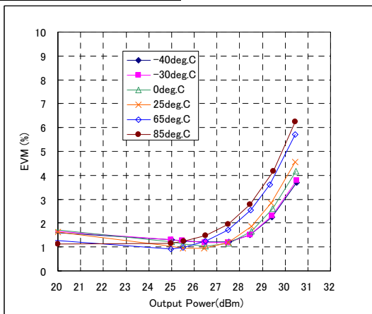
EVM vs. Output Power
