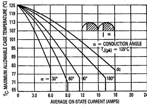
FIGURE 4 — 50-60 Hz FULL WAVE CURRENT DERATING
