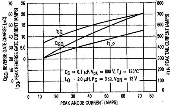
FIGURE 17 — TYPICAL TURN-OFF DYNAMICS
