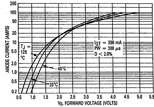
FIGURE 12 — MAXIMUM FORWARD VOLTAGE versus CURRENT
