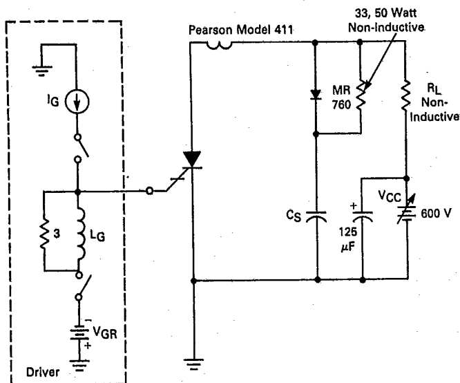
FIGURE 2 — INDUCTIVE SWITCHING TEST CIRCUIT (TURN-OFF)
