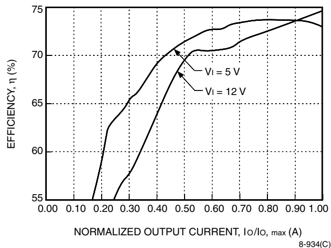
Figure 11. MH005B, C, BK, CL Typical Converter Efficiency as a Function of Output Current; T_A = 25^\circ\text{C}
