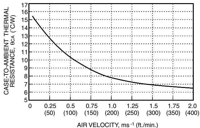
Figure 22. MH005A, B, C Case-to-Ambient Thermal Impedance
