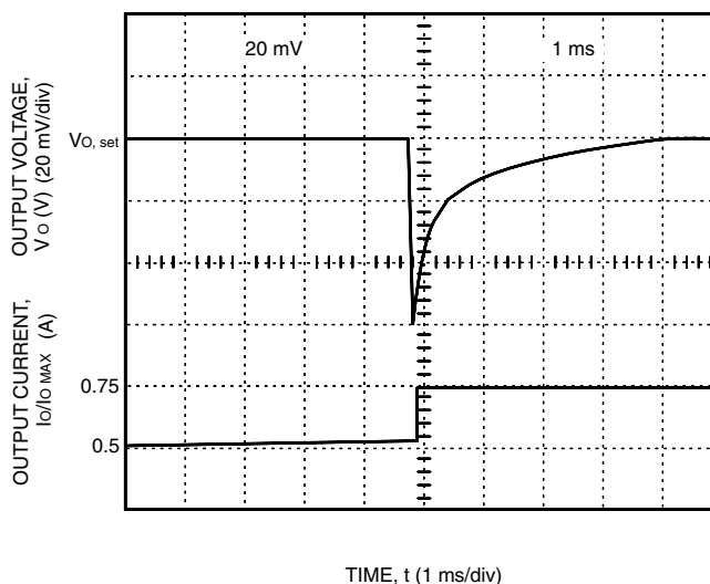
Figure 12. Typical Output Voltage for a Step Load Change from 50% to 75%
