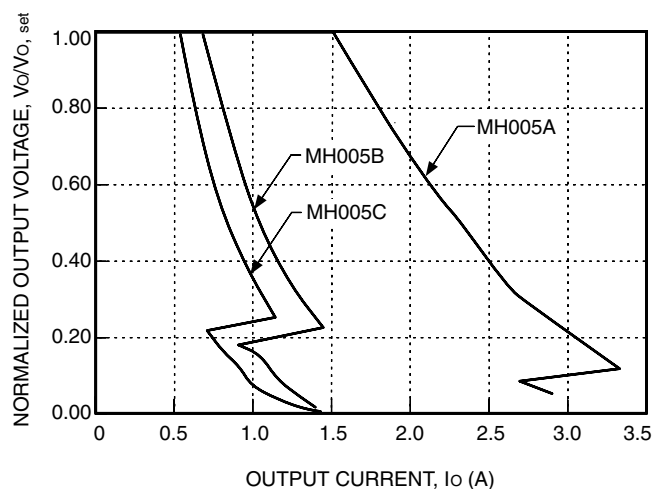
Figure 4. MH005A, B, C Typical Output Characteristics with V_i = 5\text{ V} and T_A = 25^\circ\text{C}
