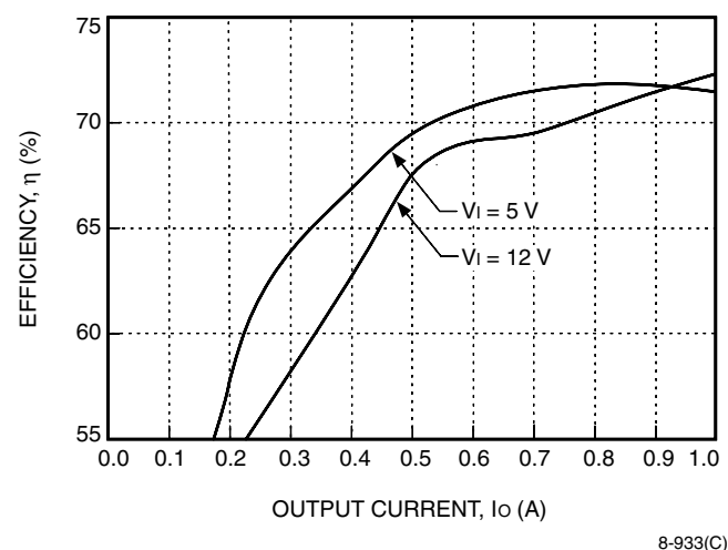
Figure 10. MH005A Typical Converter Efficiency as a Function of Output Current; T_A = 25^\circ\text{C}
