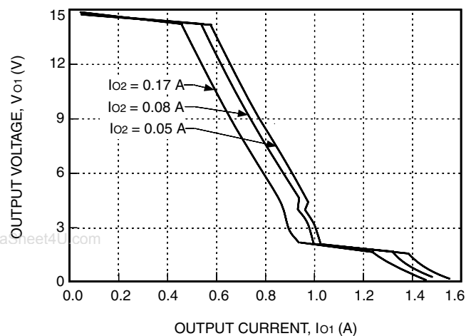
Figure 9. MH005CL Typical Output Characteristics with V_I = 12\text{ V} and T_A = 25^\circ\text{C}
