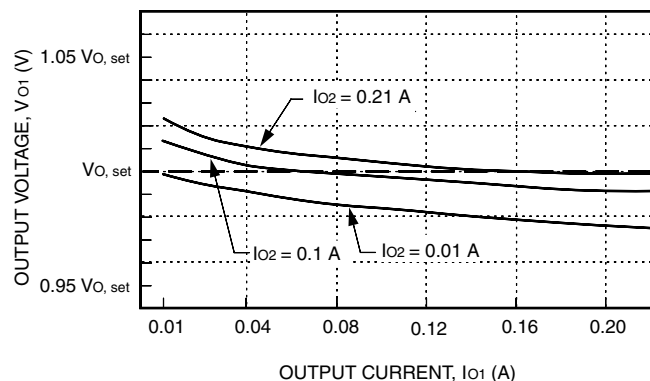
Figure 3. MH005BK, CL Typical V_o vs. I_o Regulation with V_i = 5\text{ V} and T_A = 25^\circ\text{C}
