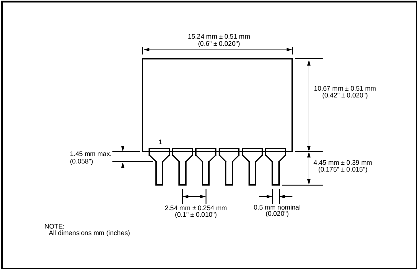
Figure 5 - Physical Dimensions
