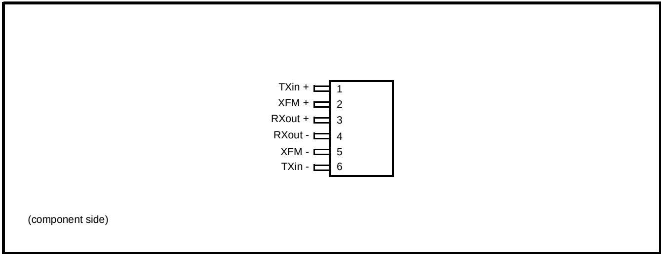
Figure 2 - Pin Connections
